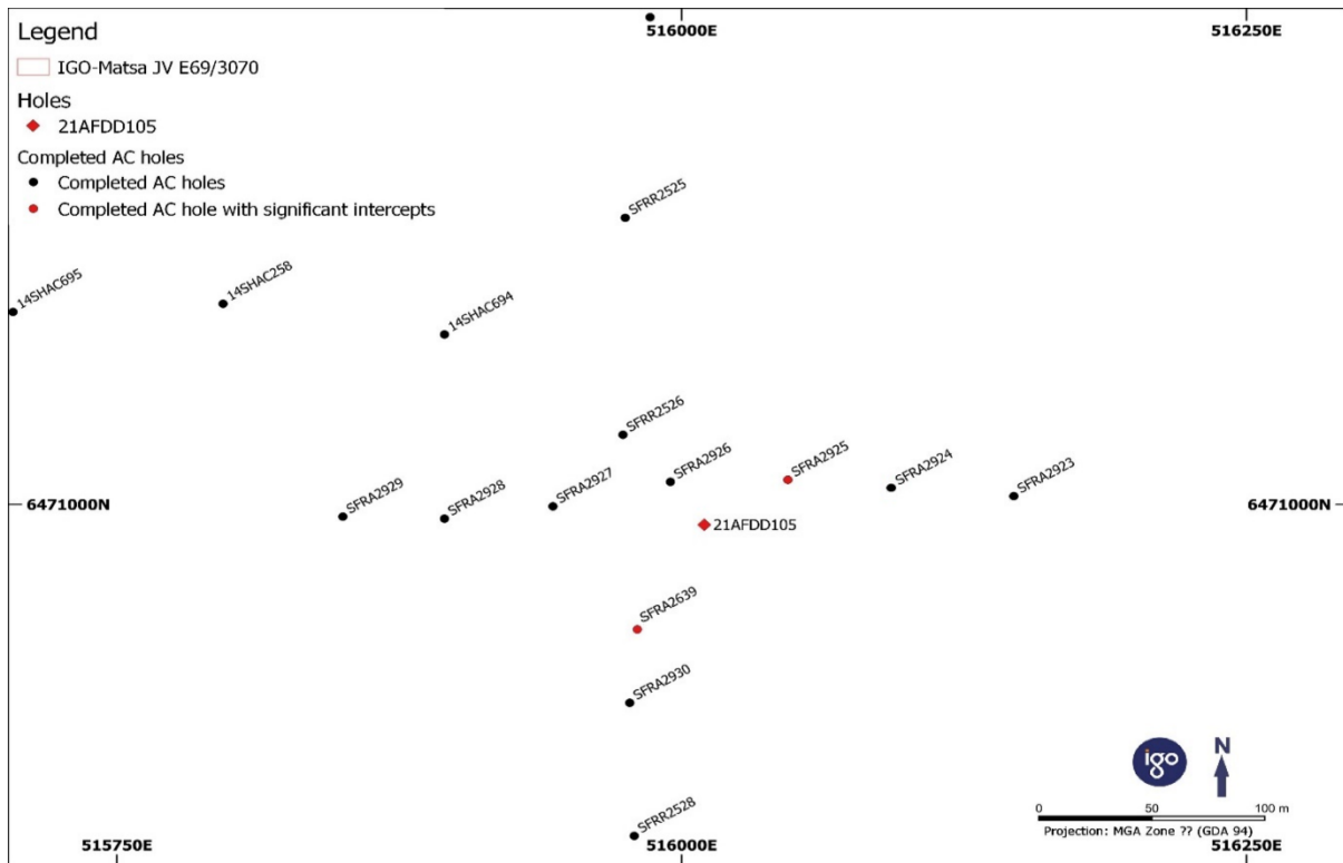
Figure 3: Plan map of 21AFDD105 and previously drilled air core (AC) holes 1
