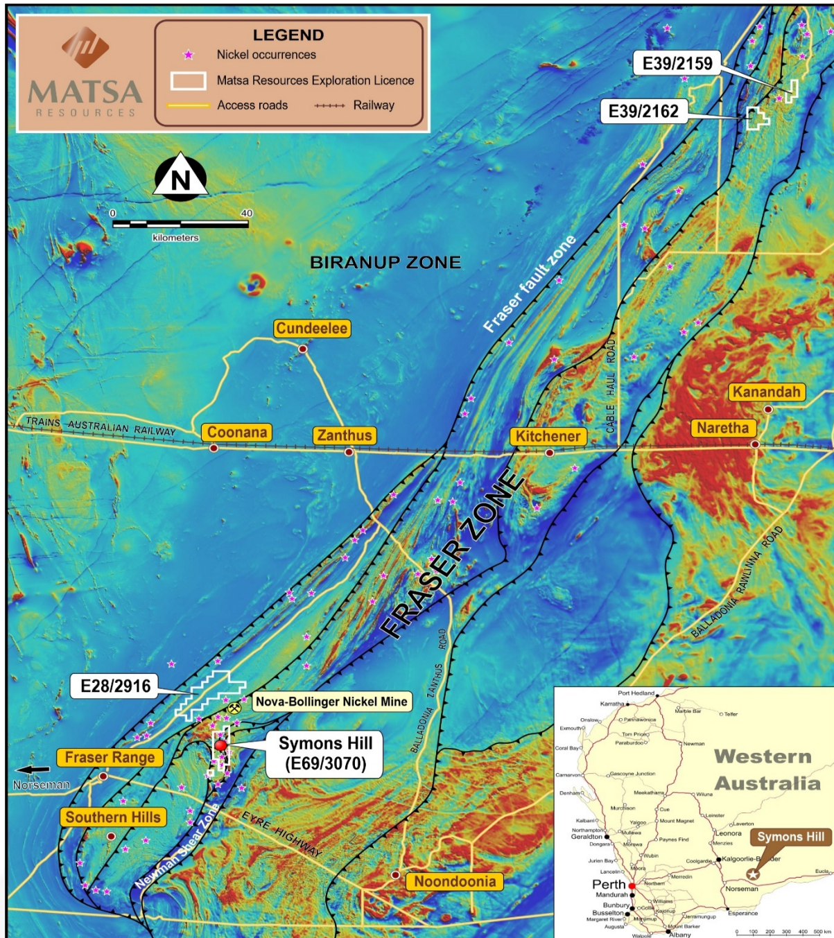
Figure 2: Matsa tenements over magnetics of the Fraser Range
