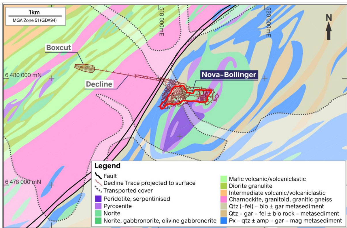
Figure 20: Nova-Bollinger infrastructure and simplified regional geology
