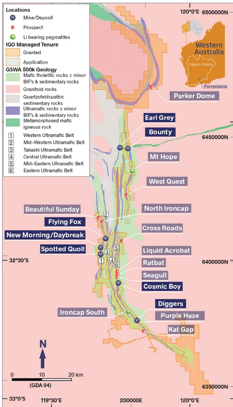
Figure 22: Forrestania simplified geology nickel and lithia deposits
