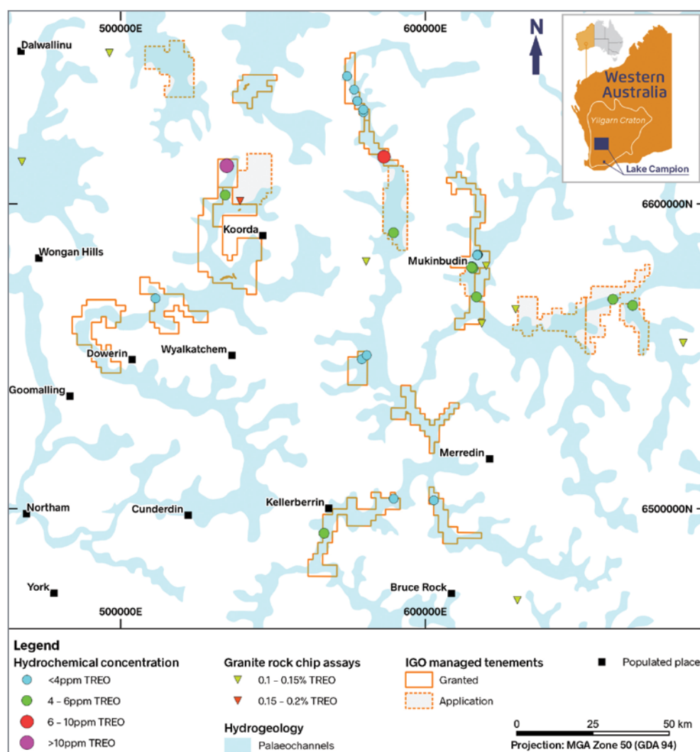
Figure 45: Lake Champion hydrogeochemical and rock chip assay REE data from the Lake Champion Project
