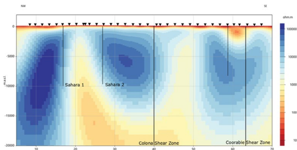
Figure 33: Sahara-Firefly MT traverse two-dimensional resistivity section to 20km depth
