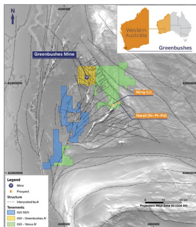
Figure 20: Greenbushes brownfields exploration tenements
