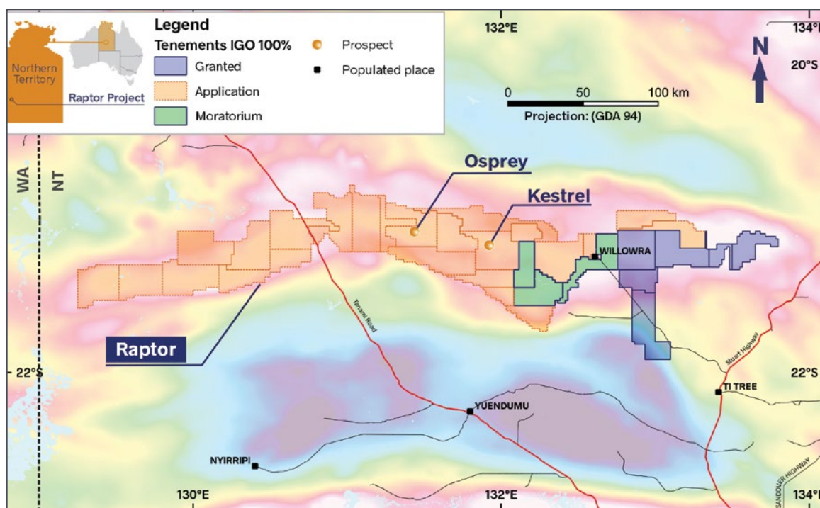
Figure 35: Raptor Project tenure over gravity image highlighting the Willowra Gravity Ridge
