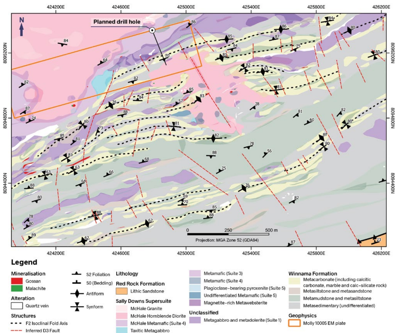
Figure 27: Osmond Valley CY22 exploration work at Molly
