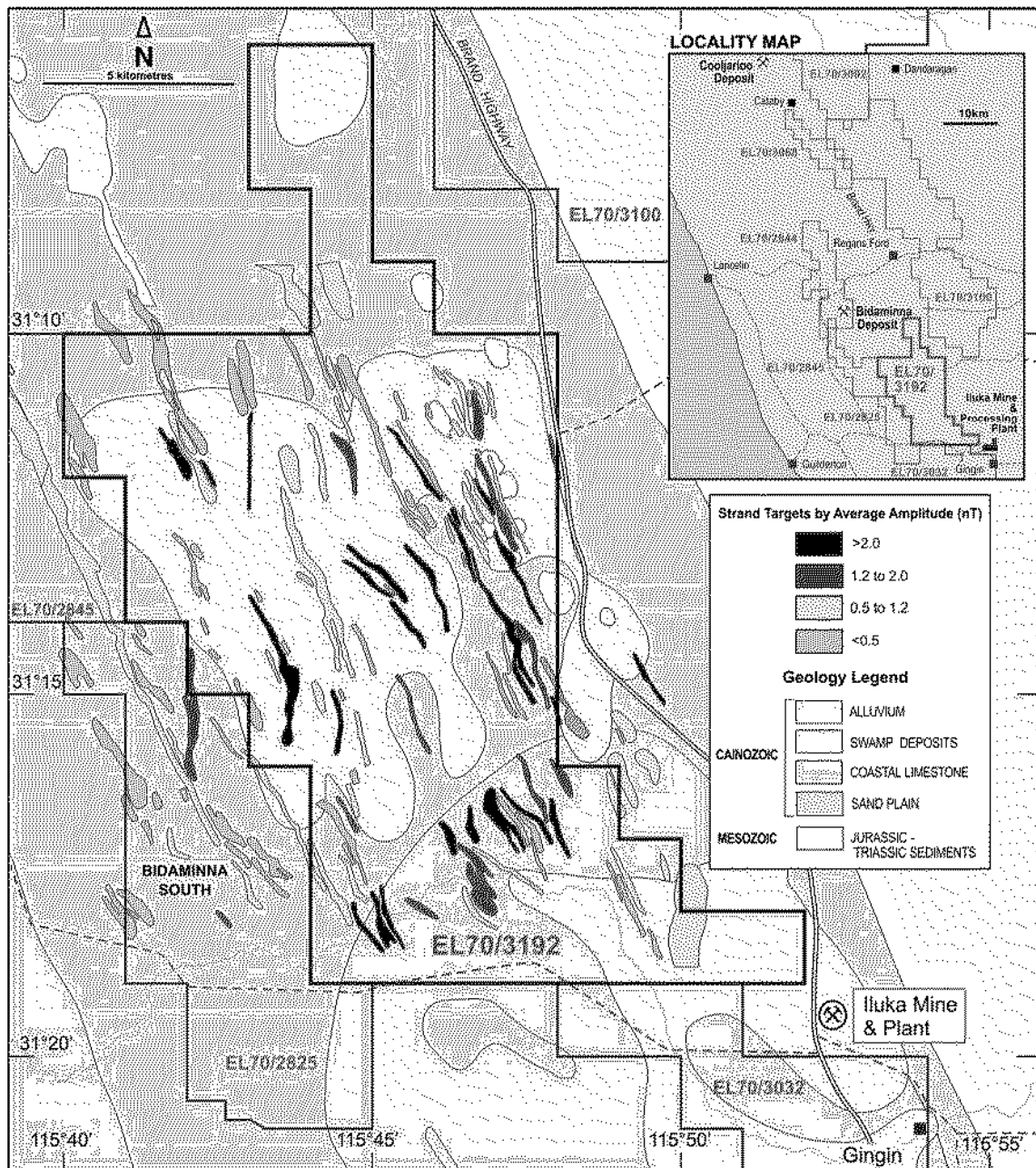
Bootine Prospect - Aeromagnetic Interpreted Strandlines
