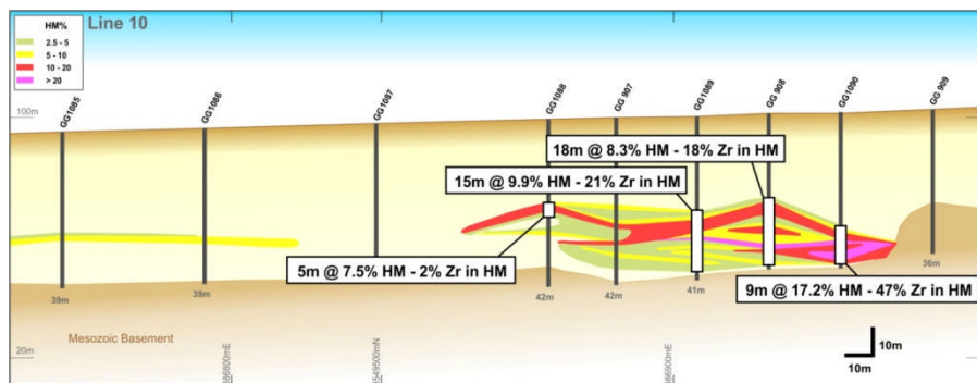
Figure 4. Section on Line 10 (refer Figure 1 for location)
