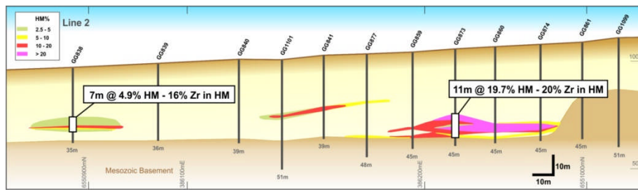
Figure 2. Section on Line 2 (refer Figure 1 for location)
