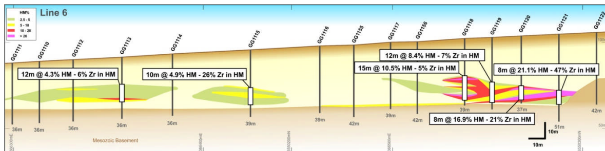
Figure 3. Section on Line 6 (refer Figure 1 for location)
