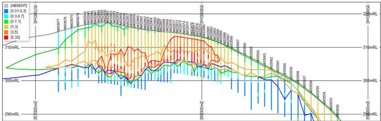
Figure 2: Cross-section (x 20 vertical exaggeration) along 6,754,900 mN of drillholes coloured by total HM, interpreted mineralised domains (0.7% total HM – green, 3% total HM – red), contains indurated material with iron staining (orange) and base of aeolian sediments (blue)
