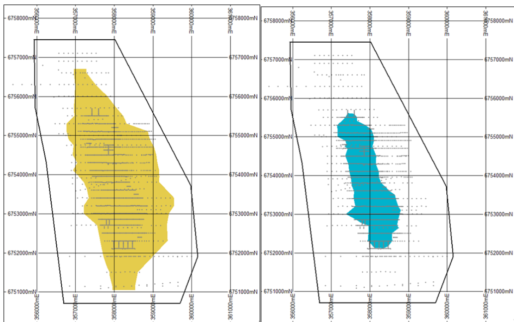
Figure 4: Yandanooka – plan of drillhole locations and mineralised domains interpreted using a nominal cut-off grades of 0.7% total HM (left half) and 3% total HM (right half)
