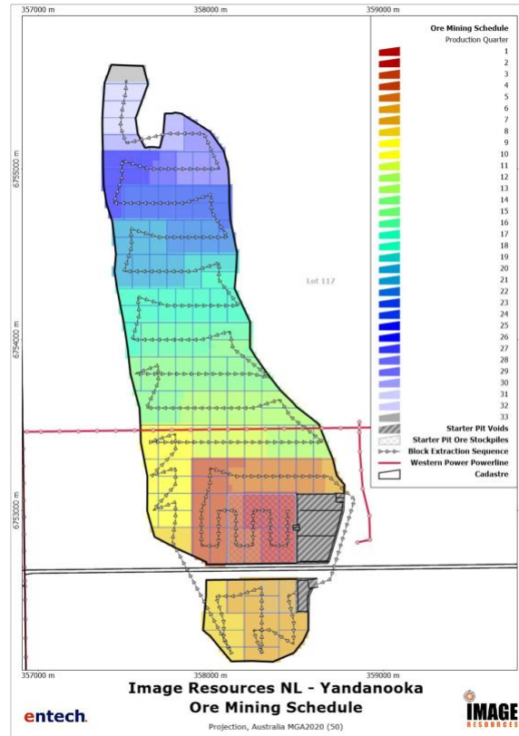
Figure 7: Mining Schedule and Sequence
