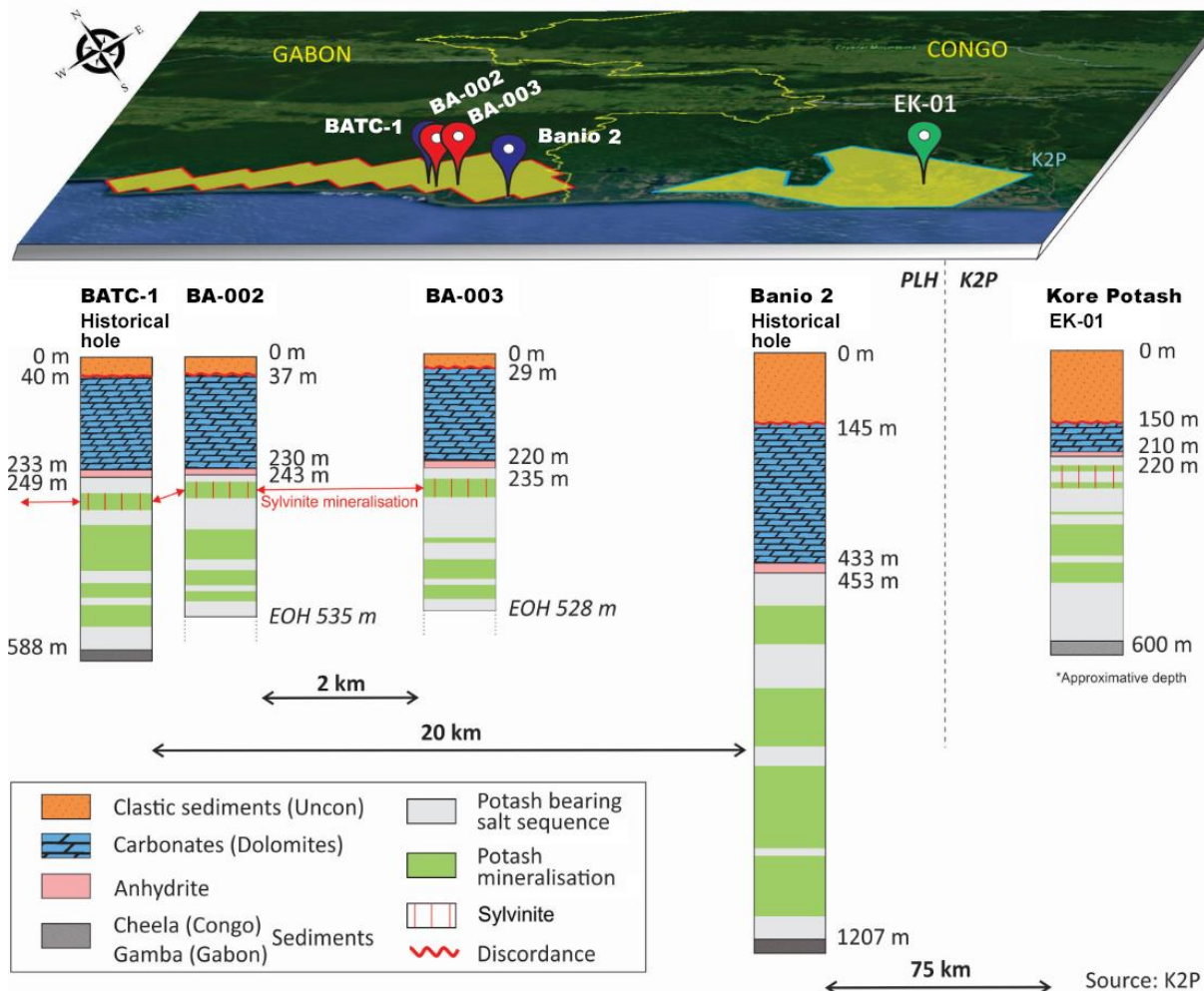
FIGURE 2: A STYLED CROSS SECTION SHOWING STRATIGRAPHIC COLUMNS OF DRILLING AND CONTINUITY ALONG A LARGE AREA IN THE CONGO BASIN
