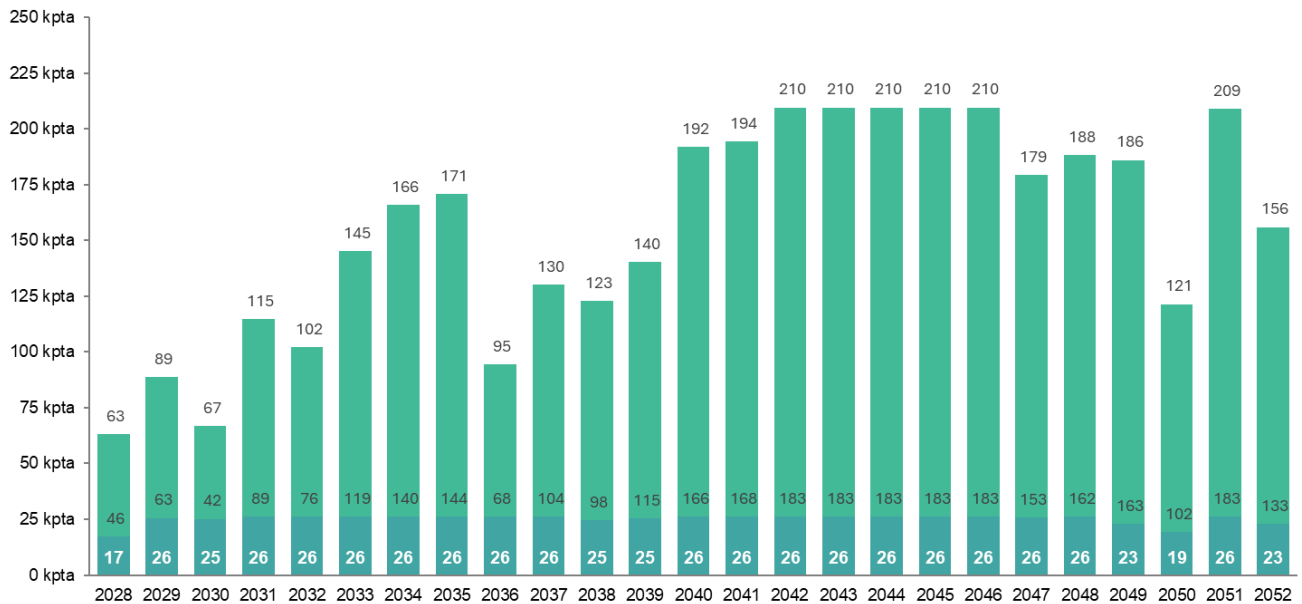
Figure 2. Lithium Carbonate Equivalent and Boric Acid Production years 1-25
