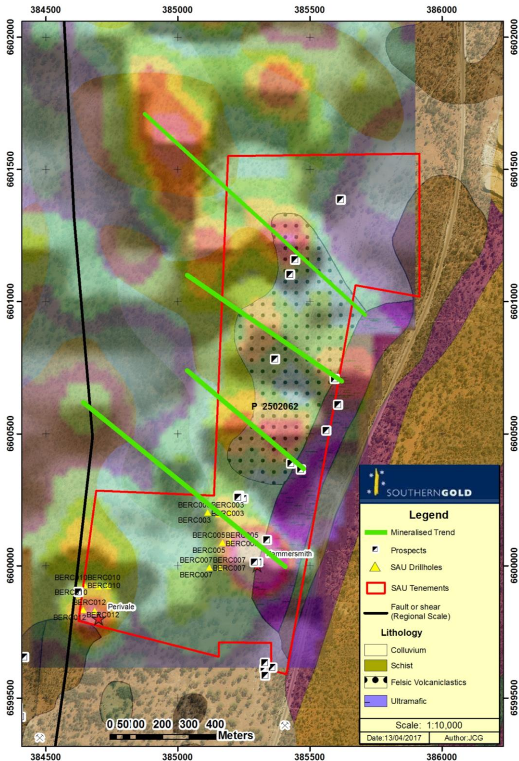
Figure 4: Hammersmith/Perivale Geochemistry
