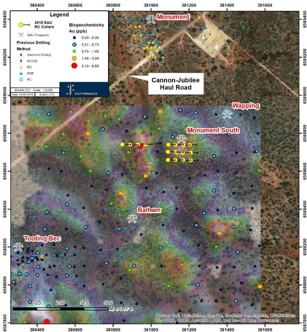
Figure 12: Plan of biogeochemical anomalism at the Monument and Tooting Bec prospects. Grid values were calculated from the individual point show.
