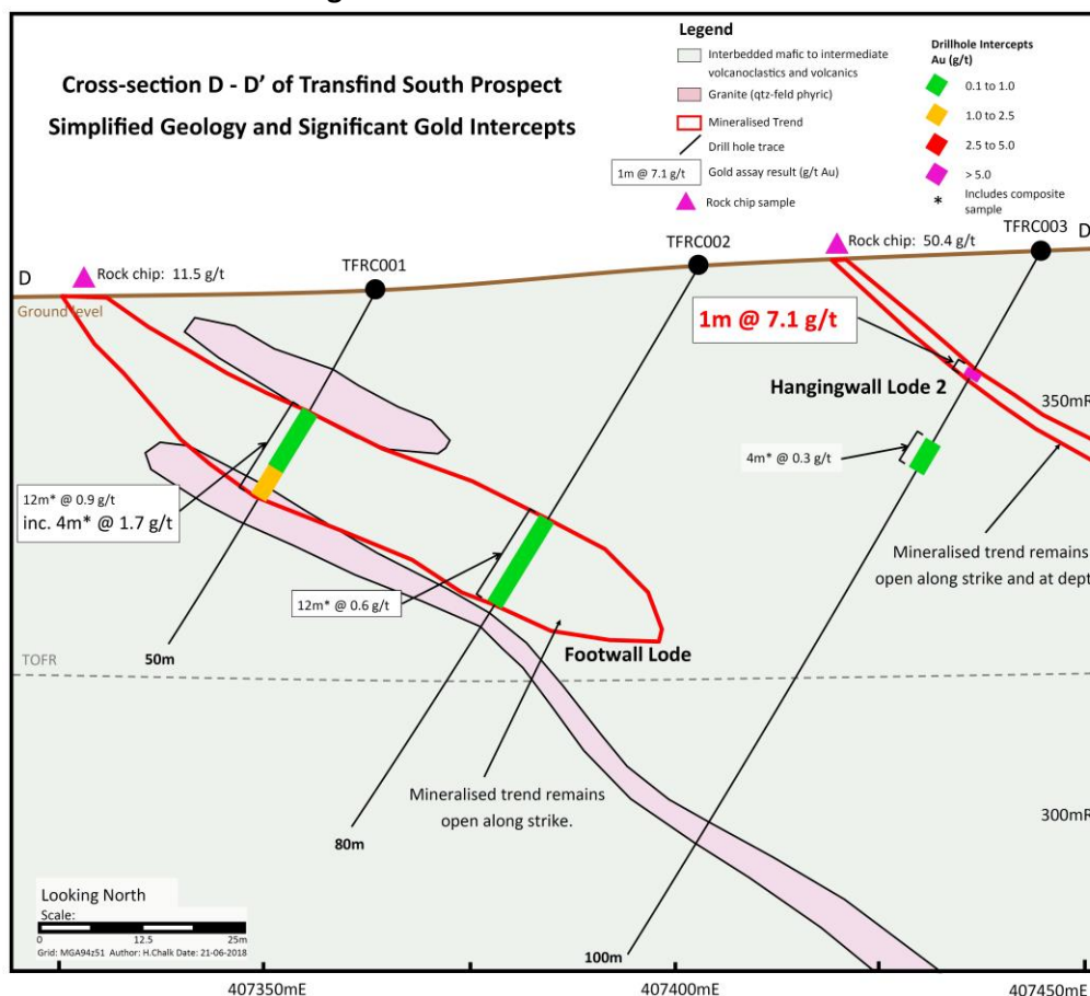
Figure 6: Cross-section 6 581 980mN.
