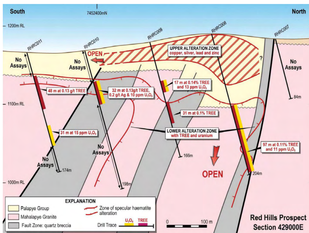
Figure 7: Cross-section through Red Hills along Traverse 429,000 mE. The Upper Zone and Lower Zone of the alteration system.
