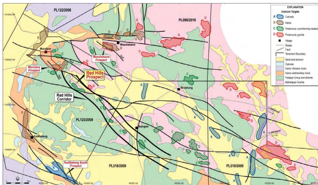
Figure 3: Surface geology of the Mahalapye area showing the Red Hills Prospect and other radiometric anomalies that are untested.
