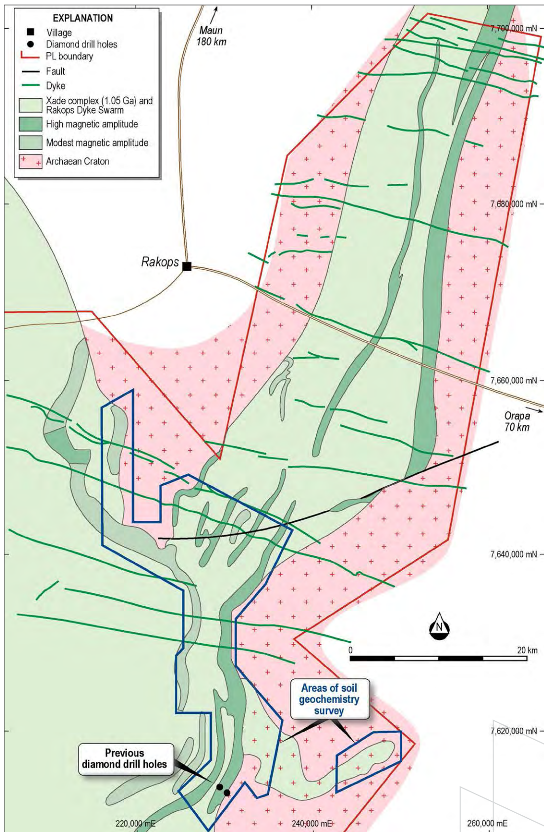
Figure 8: Bedrock geology of the northern part of the Xade Project.
