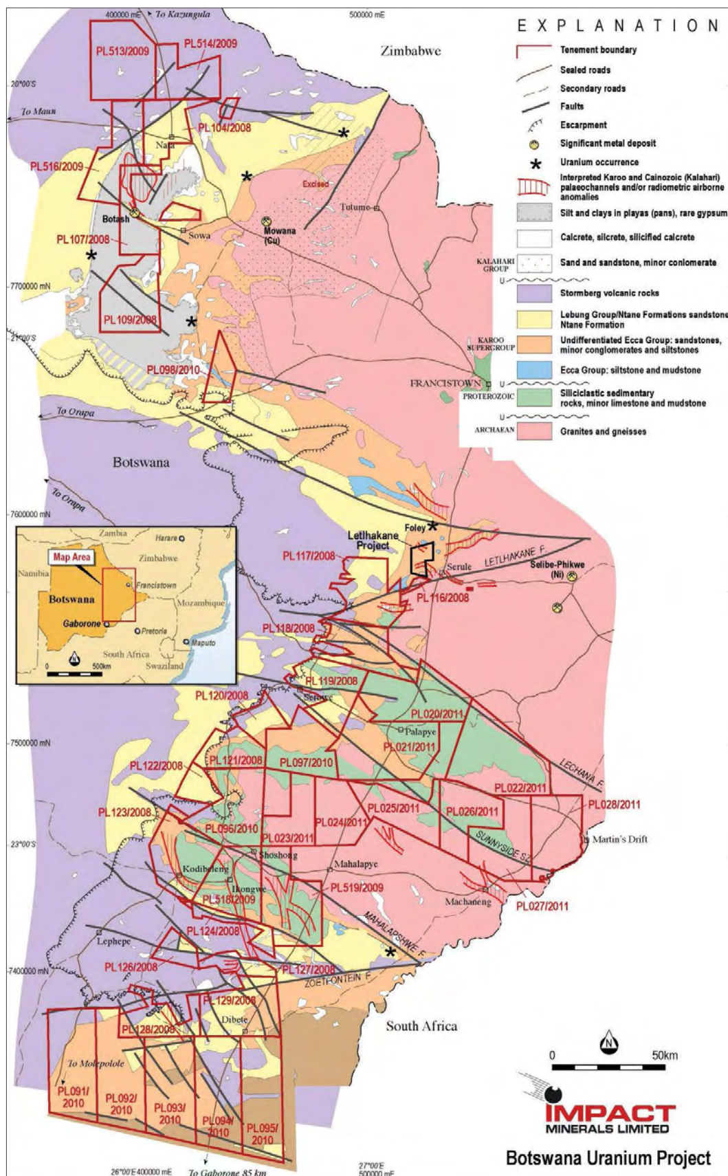
Figure 2: Geology of the Botswana Uranium Project
