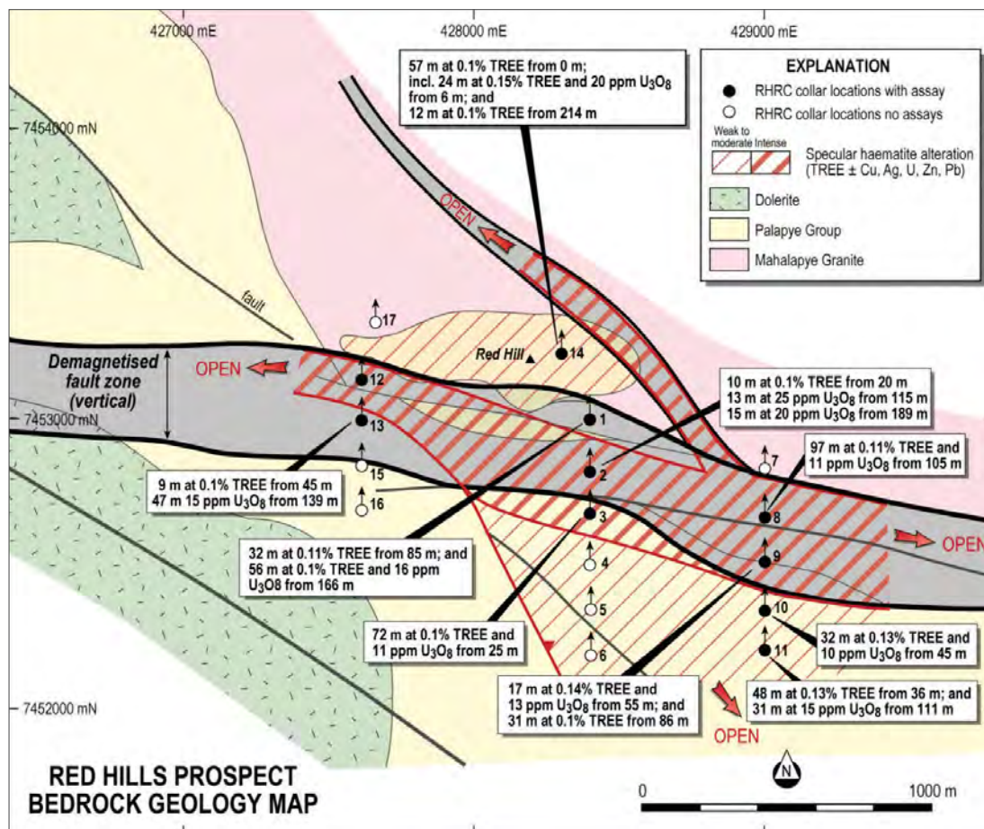
Figure 6: The geology and alteration system at the Red Hills Prospect.
