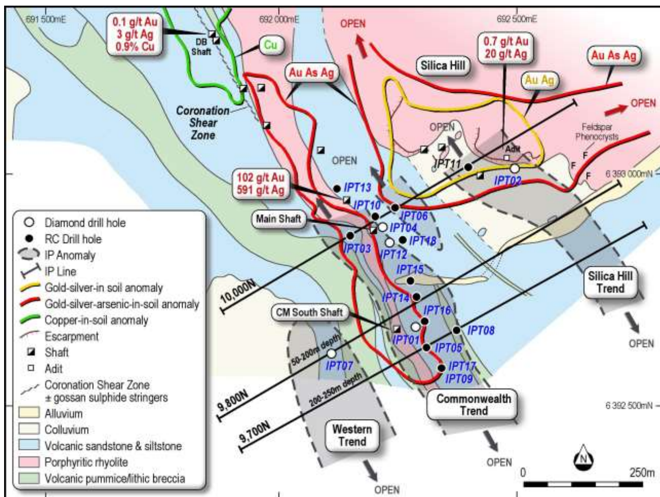
Figure 2. Geology of the Commonwealth area showing drill holes completed so far and the location of the IP Survey Lines and soil geochemistry results.
