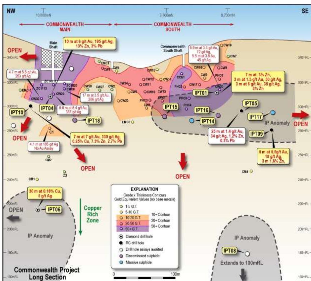
Figure 1. Long Section between Main Shaft and Commonwealth South Prospects showing the location of Impact's drill holes, previous drill holes, significant gold and silver mineralisation, IP anomalies and new drill intercepts in yellow boxes.
