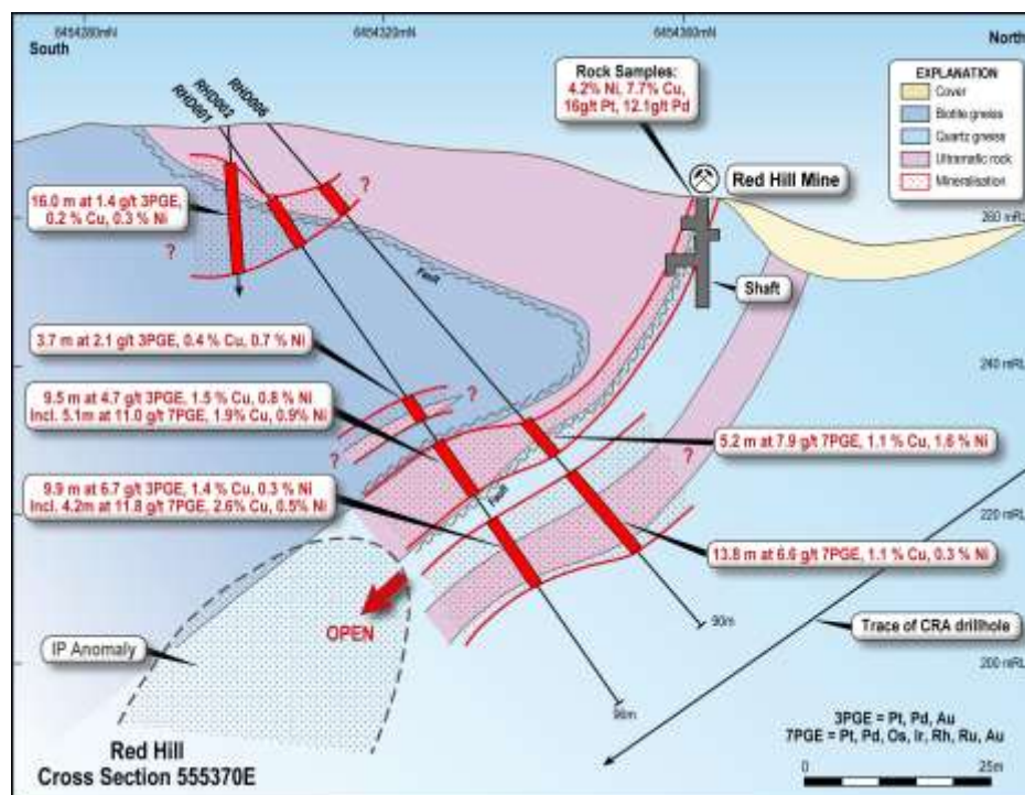
Figure 1. Cross section at the Red Hill Mine (see Figure 3 for location)
