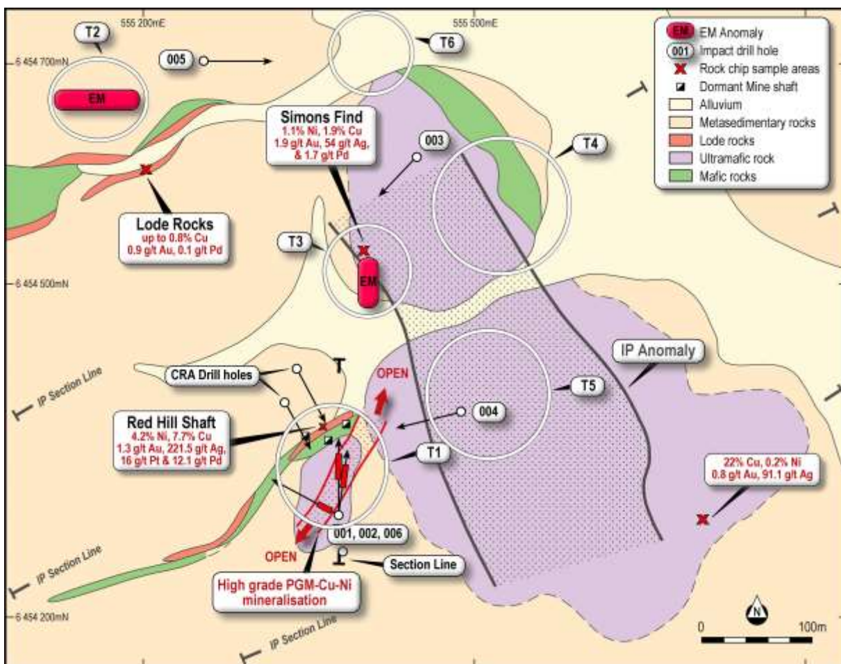
Figure 3. Geology and drill targets at the Red Hill Prospect.
