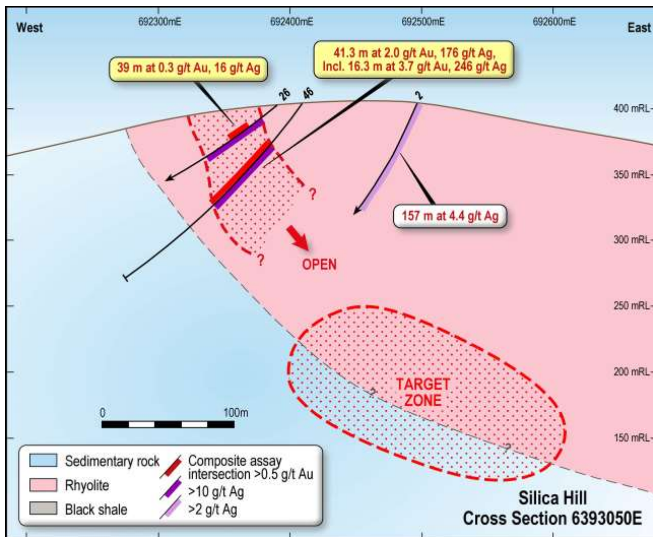
Figure 4. East-West cross section showing results for Holes CMIPT026 and 046.
