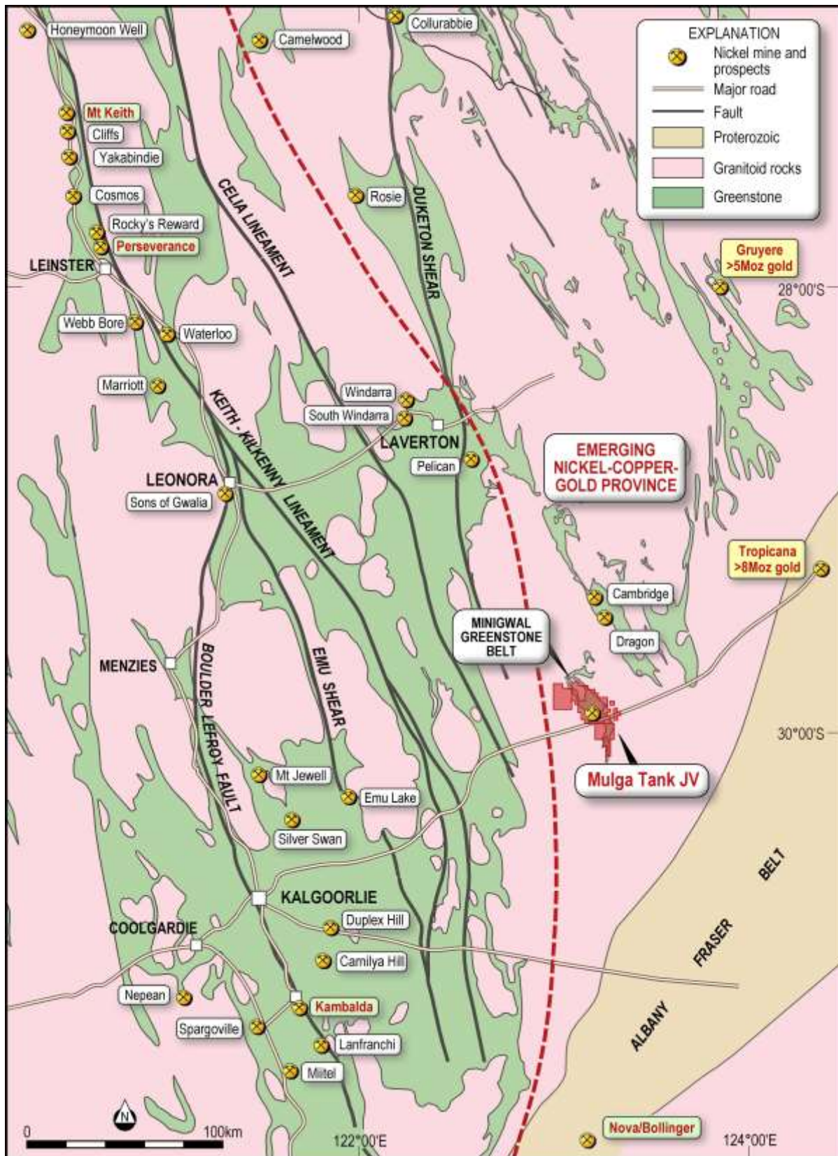
Figure 9. Location of the Mulga Tank Project and significant nickel sulphide mines and prospects including Perseverance and Rocky's Reward and with new nickel-copper-PGE discoveries in the emerging nickel-copper province to the east.
