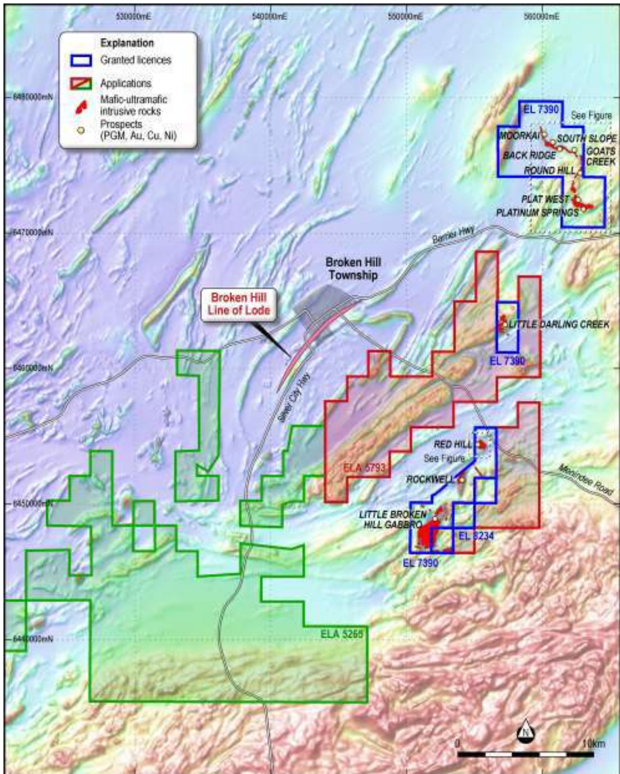
Figure 8. Impact's licences in the Broken Hill Project covering 517 square kilometres
