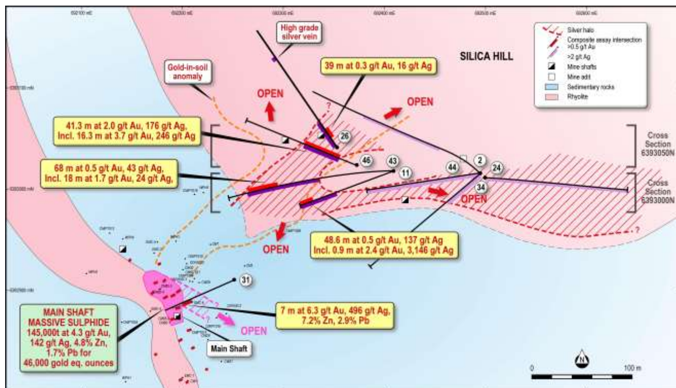
Figure 3. Surface geology map showing significant drill intercepts at Silica Hill and Main Shaft.
