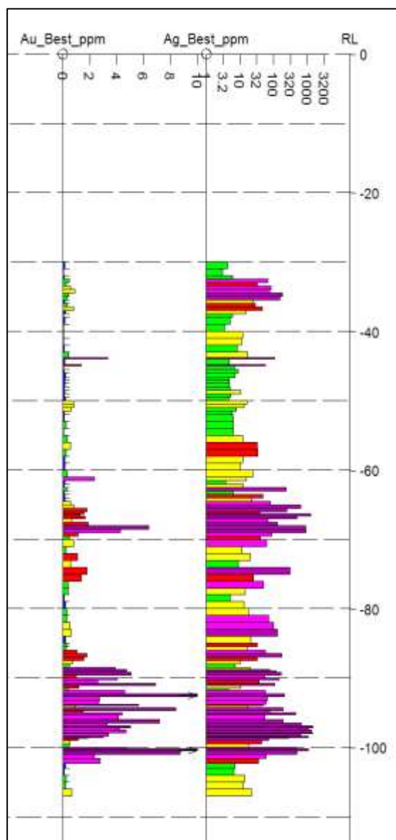
Figure 5. Detail of gold and silver assays for Hole CMIPT046. Note that the gold grades have been cut off at 10 g/t, and silver grades are at log scale to allow proper visualisation of the grades of up to 10 g/t gold and 1,490 g/t silver.
