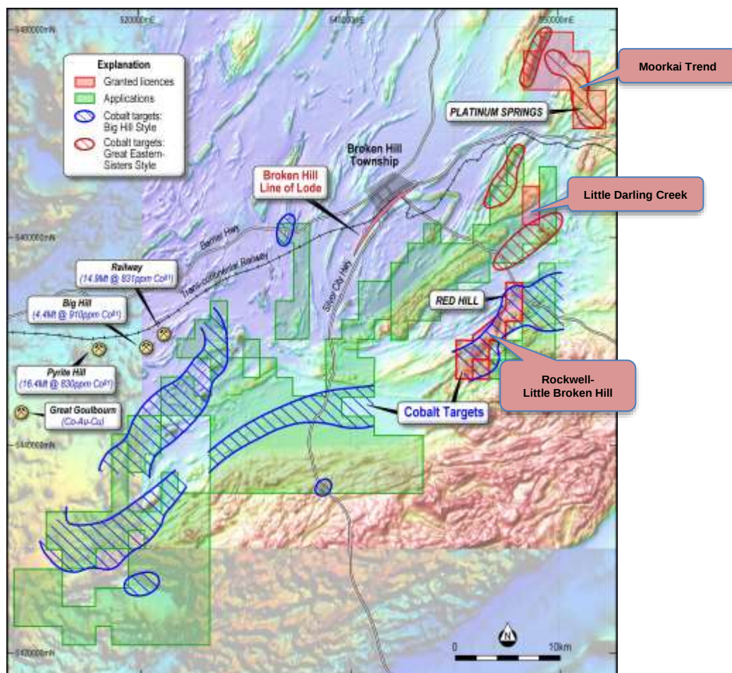
Figure 1. Image of magnetic data showing Impact's tenements at Broken Hill and key prospects.
