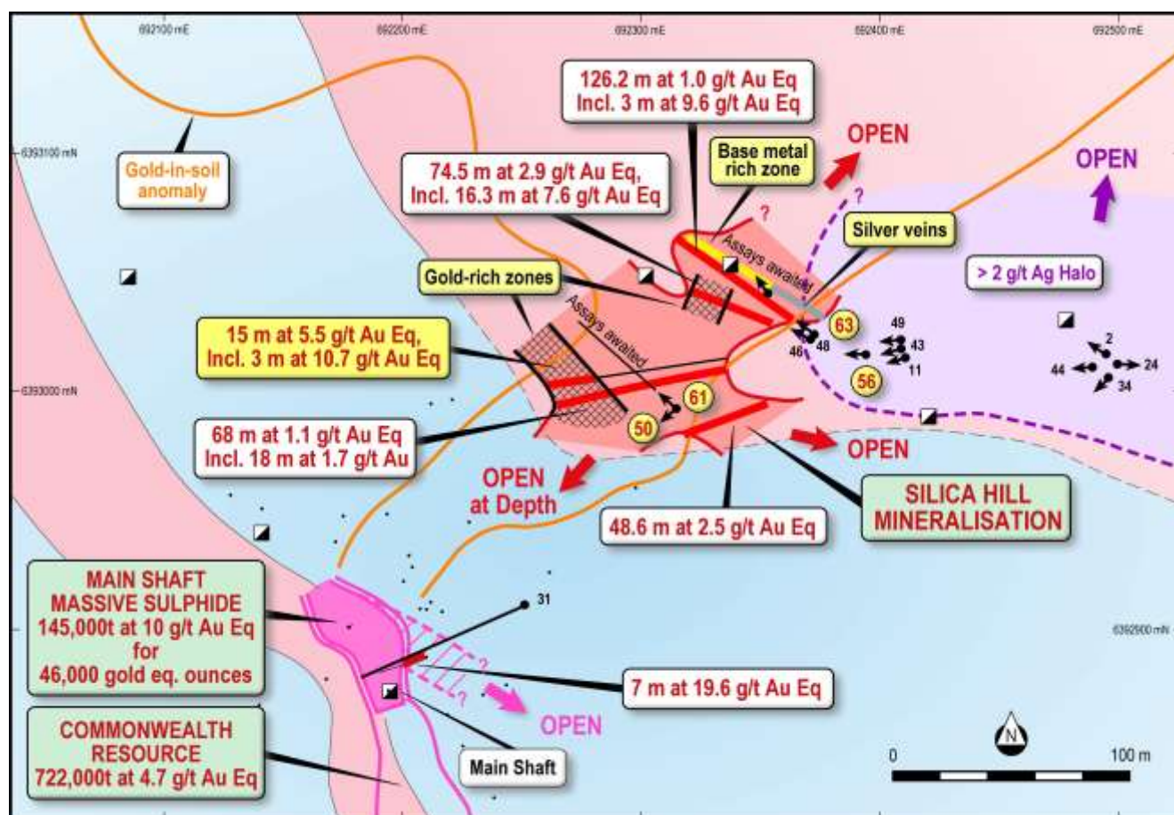
Figure 3. Significant drill results at Silica Hill. The mineralisation is open in all directions.
