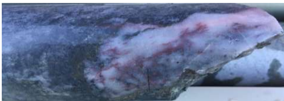
Figure 7. Quartz-ruby silver vein with pyrite and arsenopyrite from 55 m depth in Hole 61.
