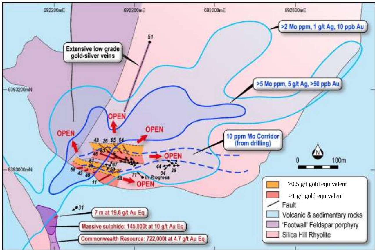
Figure 8. Overview of the Silica Hill Prospect showing drill hole locations and east-west trending gold-rich zones within a north east trending corridor defined by a gold-silver-molybdenum-in-soil anomaly. Note that the drilling has only tested the near surface portion of 10% of the target area.
