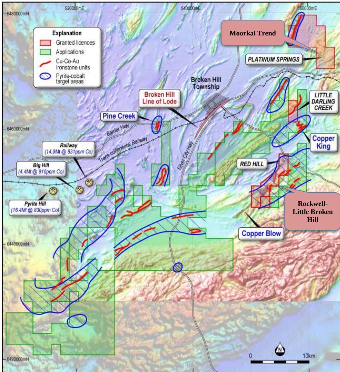
Figure 12. Image of magnetic data showing Impact's tenements at Broken Hill and key prospects.
