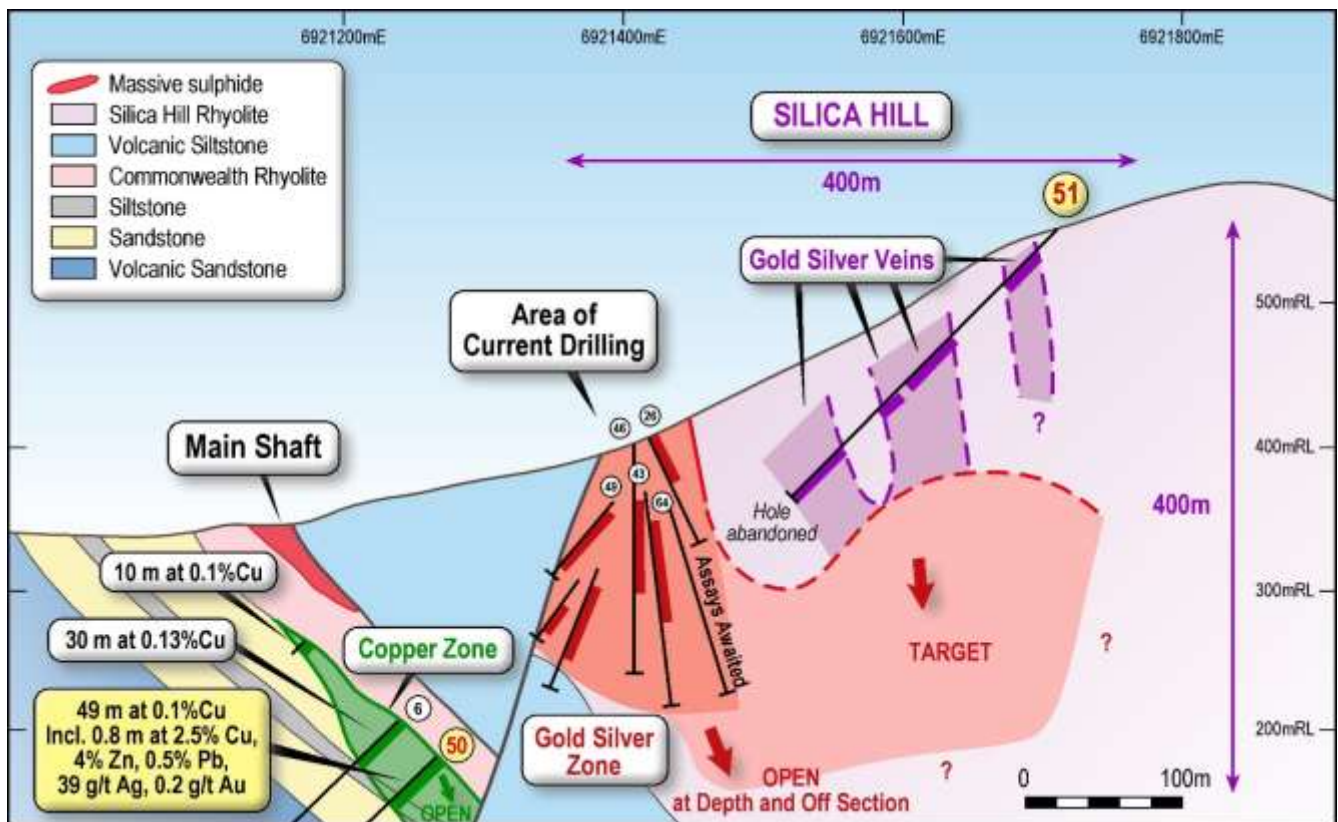
Figure 11. Cross section looking north west from Main Shaft to the south and Silica Hill to the north (see Figure 10 for location). Three components to the mineralised system are evident: an upper zone of weakly mineralised gold-silver veins; a middle zone of high grade gold-silver +/- base metal veins and a lower zone of massive sulphide and increasing copper-gold-silver at depth.
