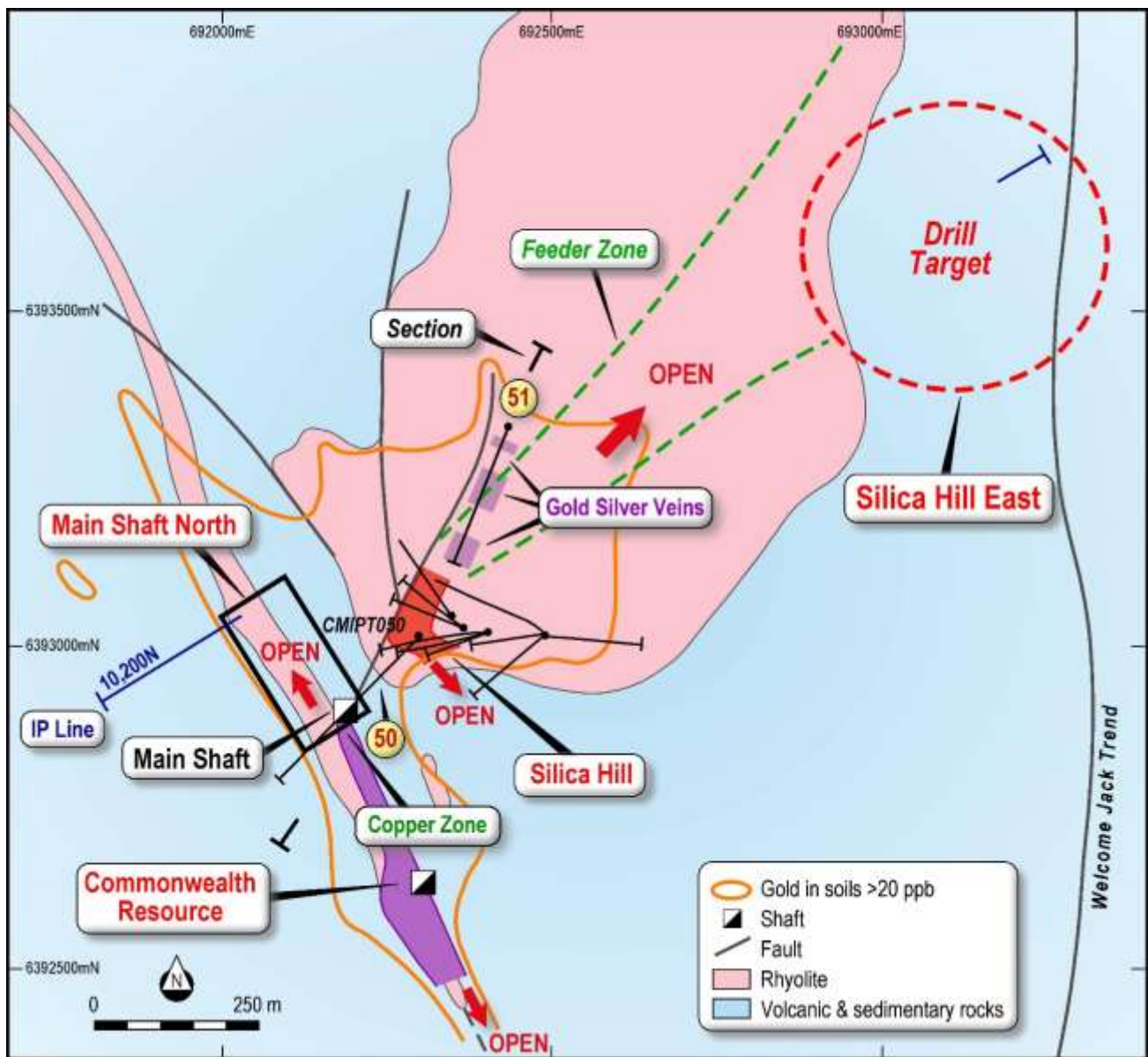
Figure 10. Geology of the Silica Hill-Commonwealth area and locations of Holes CMIPT50 and 51. Note that the low grade gold-silver veins in Hole 51, drilled from north east to south west, overlies an interpreted north east trending feeder zone. Hole 50 tested a conductor below Main Shaft and intersected a broad zone of copper sulphide mineralisation.
