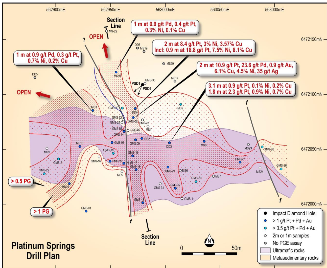
Figure 5. Geology and location of PSD01 and PSD02, previous drill holes and contoured data of previous drill assays for platinum, palladium and gold (summed from down hole intervals).
