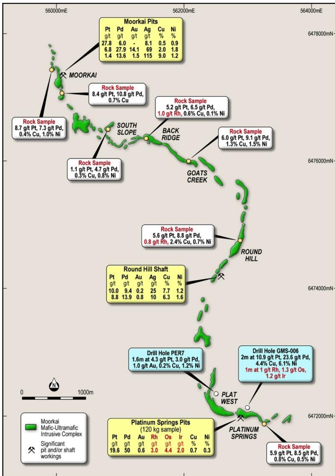
Figure 2. Rock chip samples results from along the Moorkai Trend.
