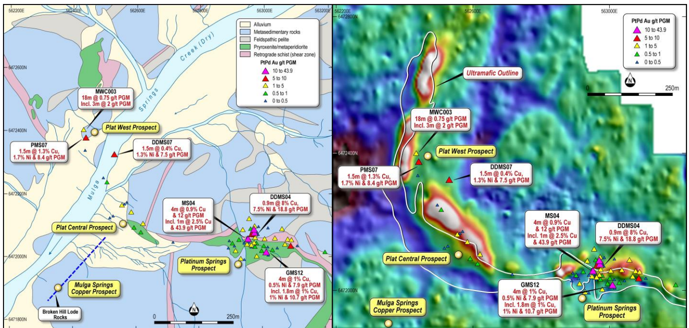
Figure 3 and 4. Surface geology (left) and image of magnetic data (right) of the Platinum Springs area showing key prospects and previous drill results.
