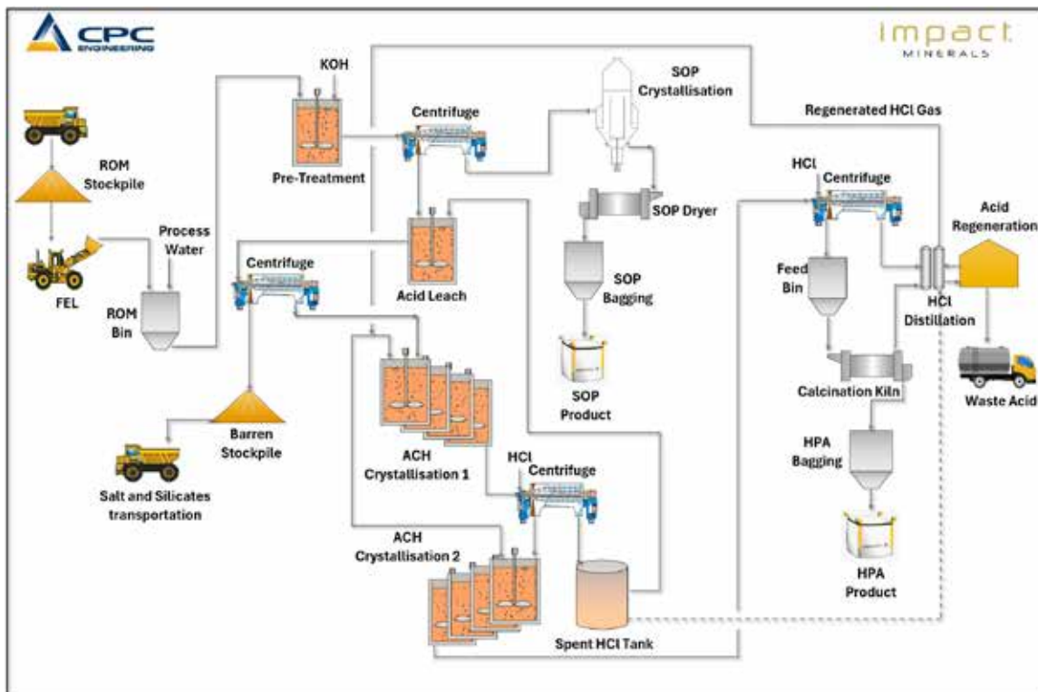
Figure 1.6. Process Flowsheet for production of HPA.
