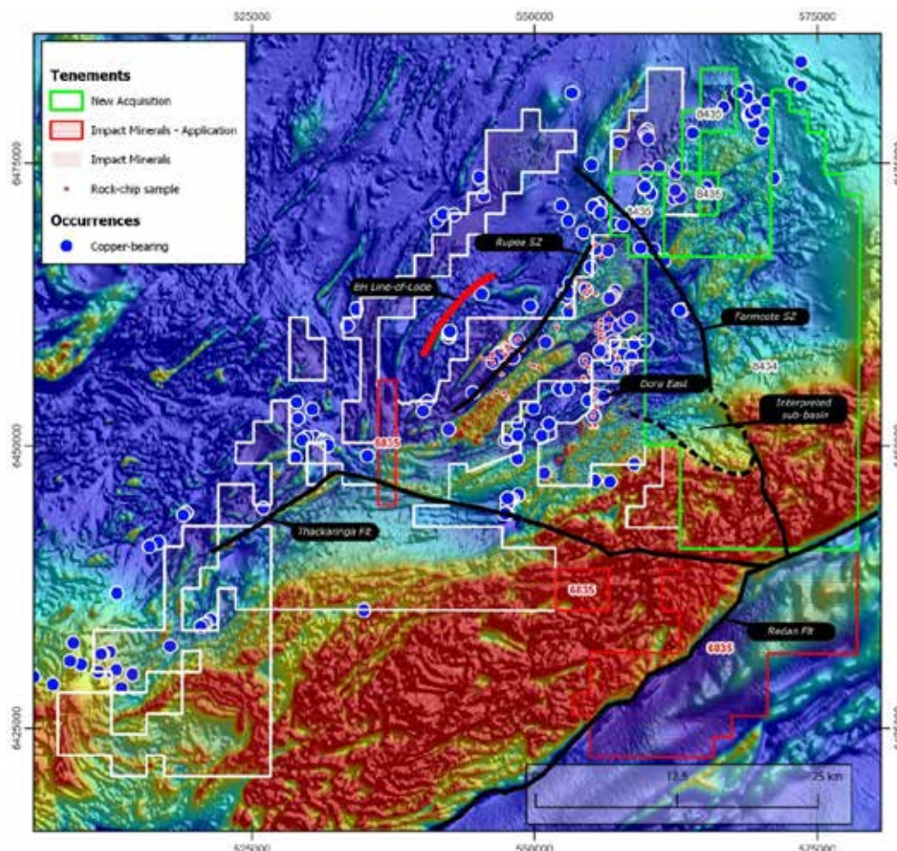
Figure 3.1. Image of regional total magnetic intensity showing the Broken Hill orebody (Line of Lode), Impact's granted licences and licence applications and the new tenements acquired. Note the Thackaringa Fault and Farmcote shear zone, both interpreted as deep-seated long-lived crustal lineaments, and the interpreted sub-basin in the new tenements. Widespread copper occurrences attest to the prospectivity of the region for copper. Impact's rock chip locations are also shown.
