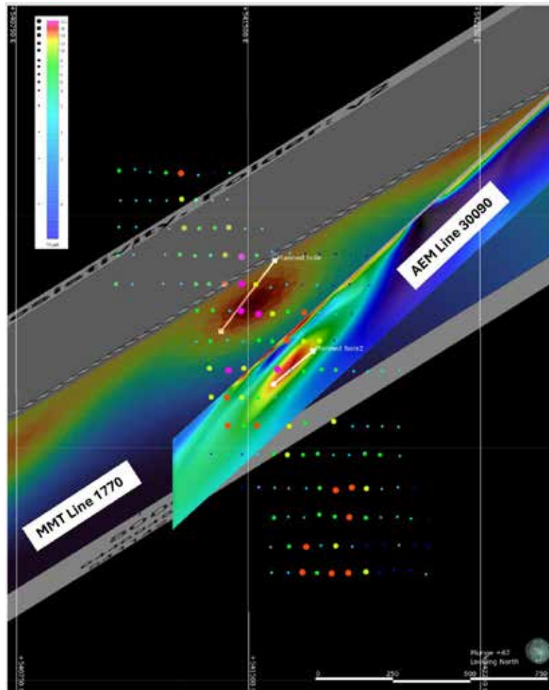
Figure 2.8. A tilted 3D view of showing the palladium-in-soil anomaly and planned drill holes to test the MMT conductor on Line 1770 and the airborne EM conductor on Line 30090.
