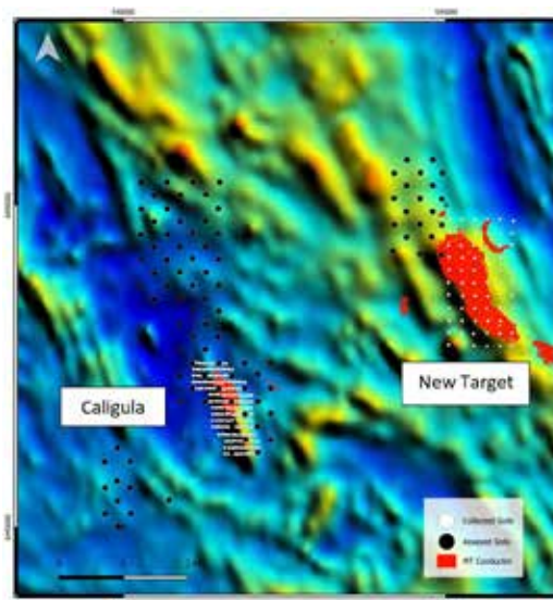
Figure 2.2. Magnetic map highlighting Mobile MT anomalies (in red) at the Caligula and New Target showing previous assayed soil sampling (black points) and new collected soil locations (white points).
