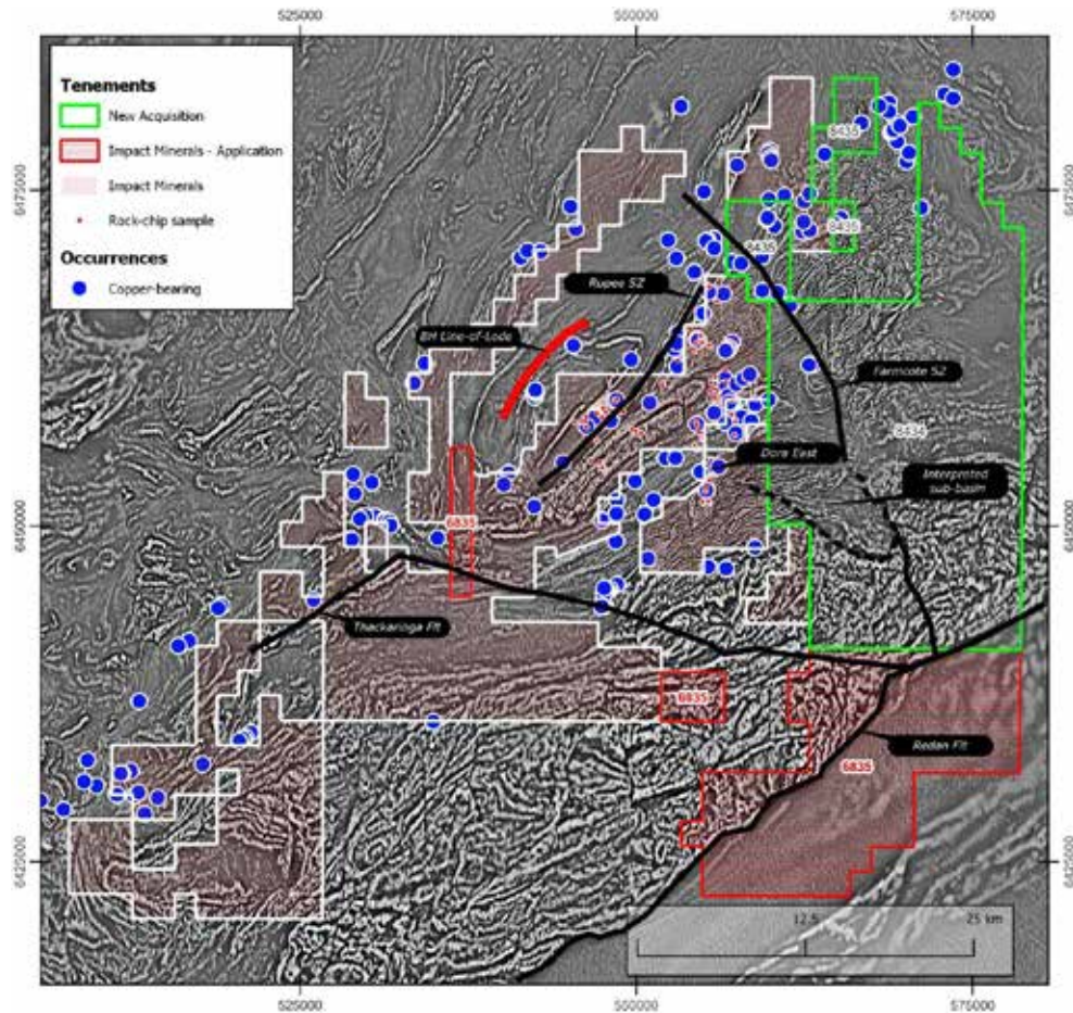
Figure 3.2. Image of the first vertical derivative of regional magnetic data as in Figure 3.1. A detailed interpretation of this data has resulted in the identification of numerous target areas for large copper deposits.
