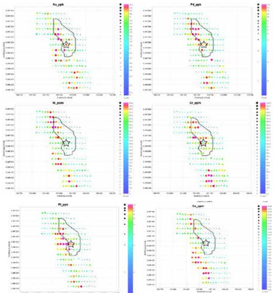
Figure 2.7. Soil geochemistry results for gold (Au)- palladium (Pd)- Platinum (Pt)- Nickel (Ni)-Chrome (Cr) and Cobalt (Co). The black outline denotes the modelled highest conductivity from the Mobile MT survey, and the Black Star is the location of an airborne EM anomaly.
