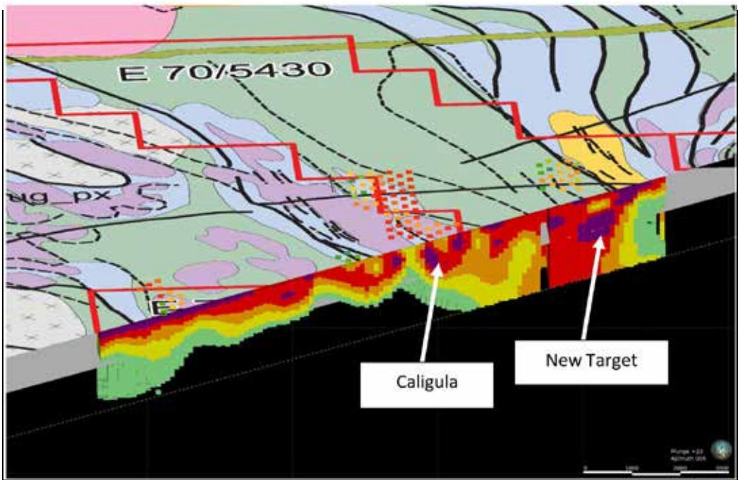
Figure 2.4. A tilted 3D view of an image of the bedrock geology of the Caligula area showing the soil geochemistry anomaly (coloured squares) and a section line of the MMT data. Purple areas are zones of high conductivity, and two such zones coincide with the geochemistry. A large conductive anomaly close to a major structure occurs at the eastern end of the section line. This is a priority area for further exploration.
