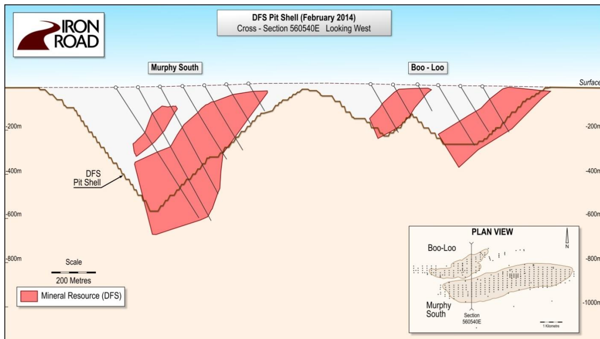
Figure 2 Cross-section through Murphy South and Boo-Loo pits as designed during the DFS (February 2014).
