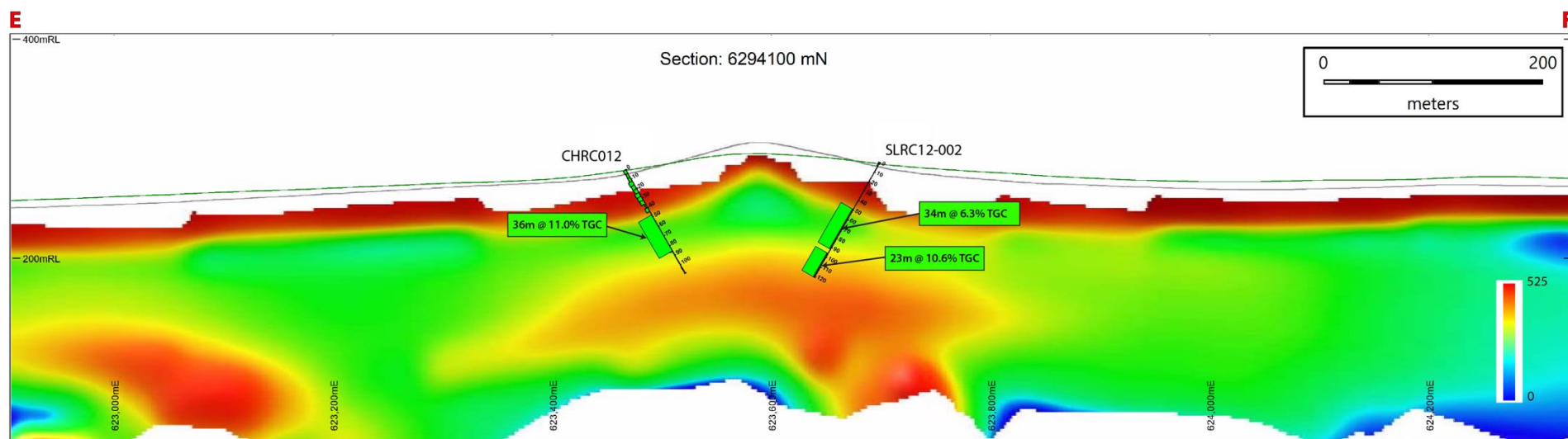
Figure 6. East-West section through the Sugarloaf Graphite Prospect – Eyre Peninsula, South Australia
