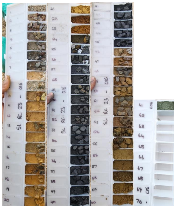
Figure 2. Chip tray photographs from hole SLRC23-016. The image shows a 37m interval of graphite mineralisation from 23m to 60m downhole. True thickness is unknown.
