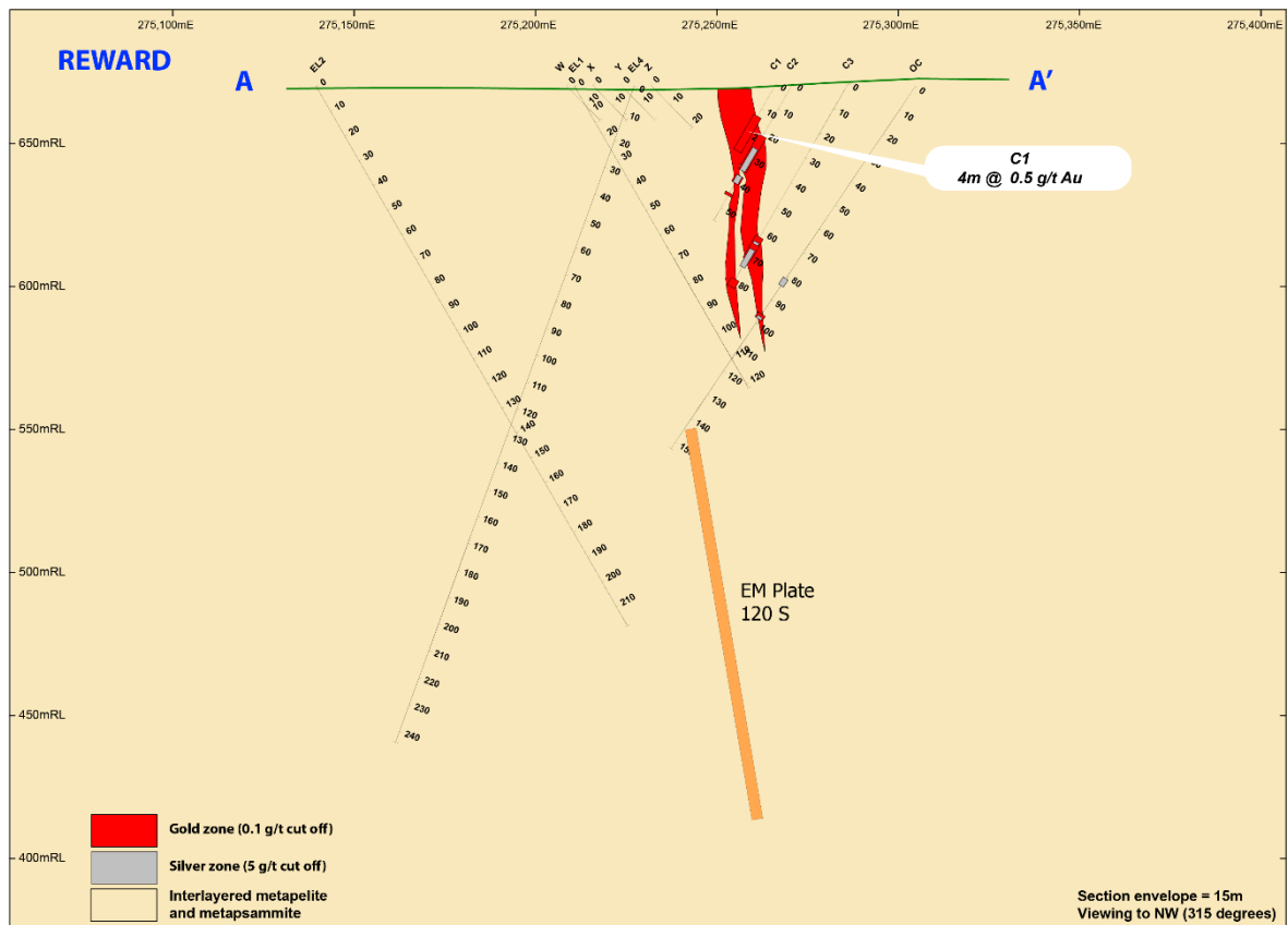
Figure 7. Section through the Reward Prospect showing drill holes with gold and silver intercepts in relation to new EM targets (ASX: ITM 7 July 2025).
