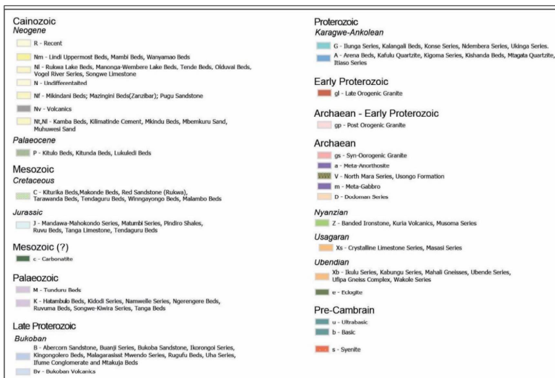
Figure 3.6: Legend for the regional geological map
