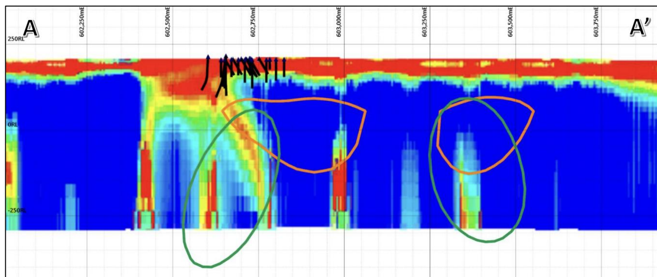
Figure 4 - Section A-A' over the Athena targets. Strong AEM conductors are seen on the periphery of the magnetic inversion shells (green shells representing 100,000 T). Current existing drillholes at Athena shown at surface. Core of magnetic shells and contacts with AEM signals currently untested as is Eastern magnetic shell. Gravity inversion modelling of bodies with density 2.77 g/cm 3 compared to average rock density of 2.67 g/cm 3 .
