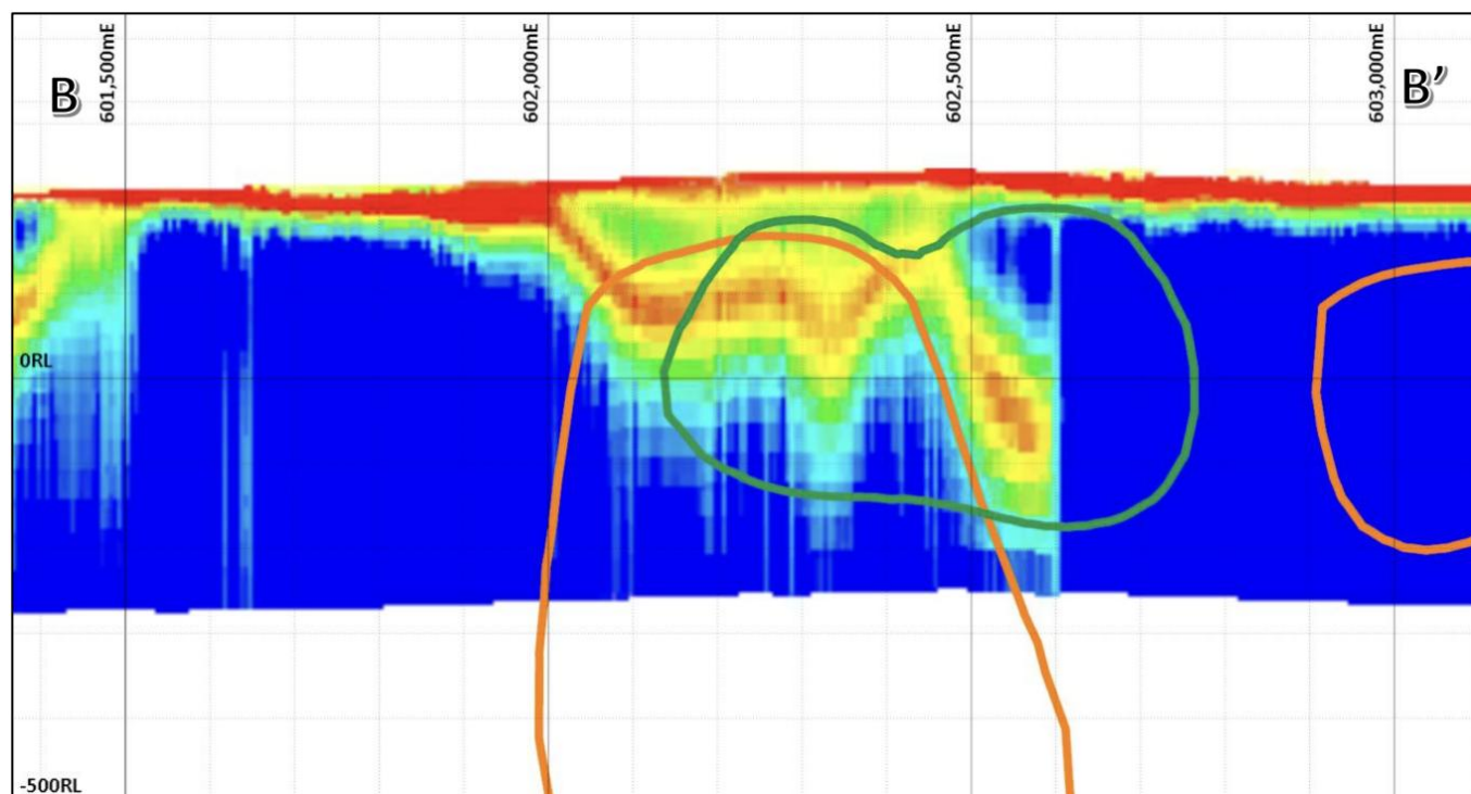
Figure 5 - Section B-B' over the Hestia Target showing strong AEM signals associated with high magnetics (green shell) and gravity anomalies
