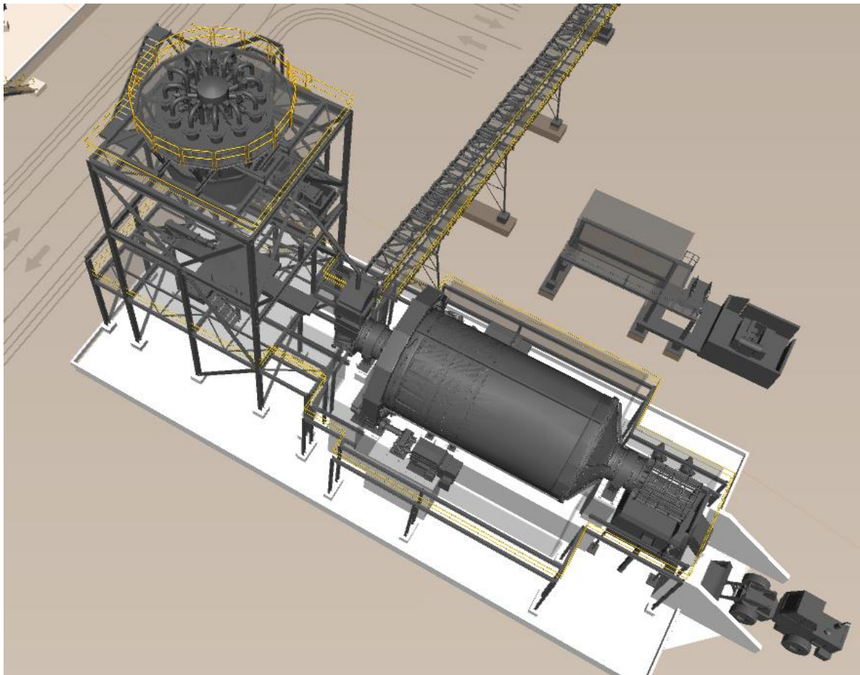
Figure 6.4 Ball Mill Grinding and Hydro-cyclone Classification
