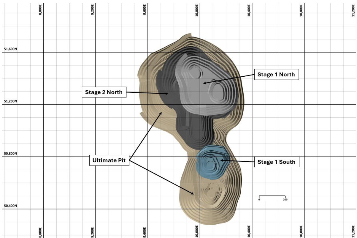
Figure 5.2 Pit stages guided by pit optimisation process (plan and isometric)
