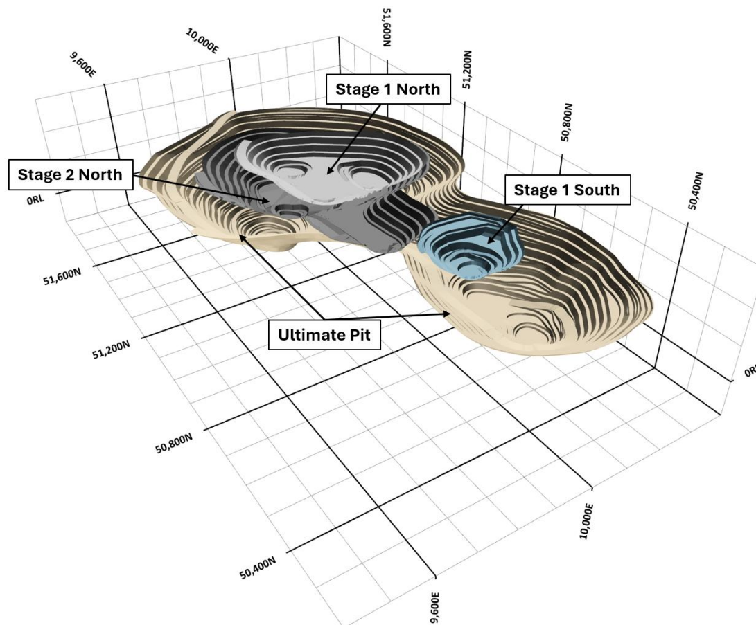
Figure 1.5 Pit stages target high grade, low strip ratio early
