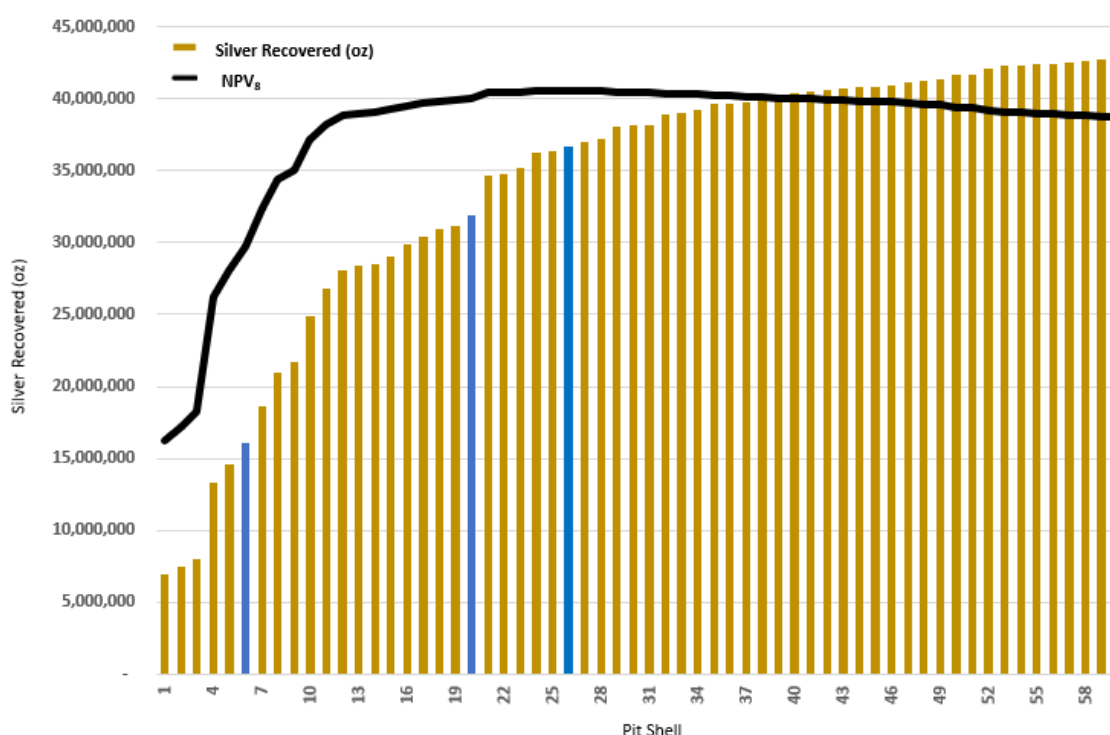
Figure 5.1 Paris Silver Pit Optimisation – recovered silver from different pit shells with shells used in pit design in blue
