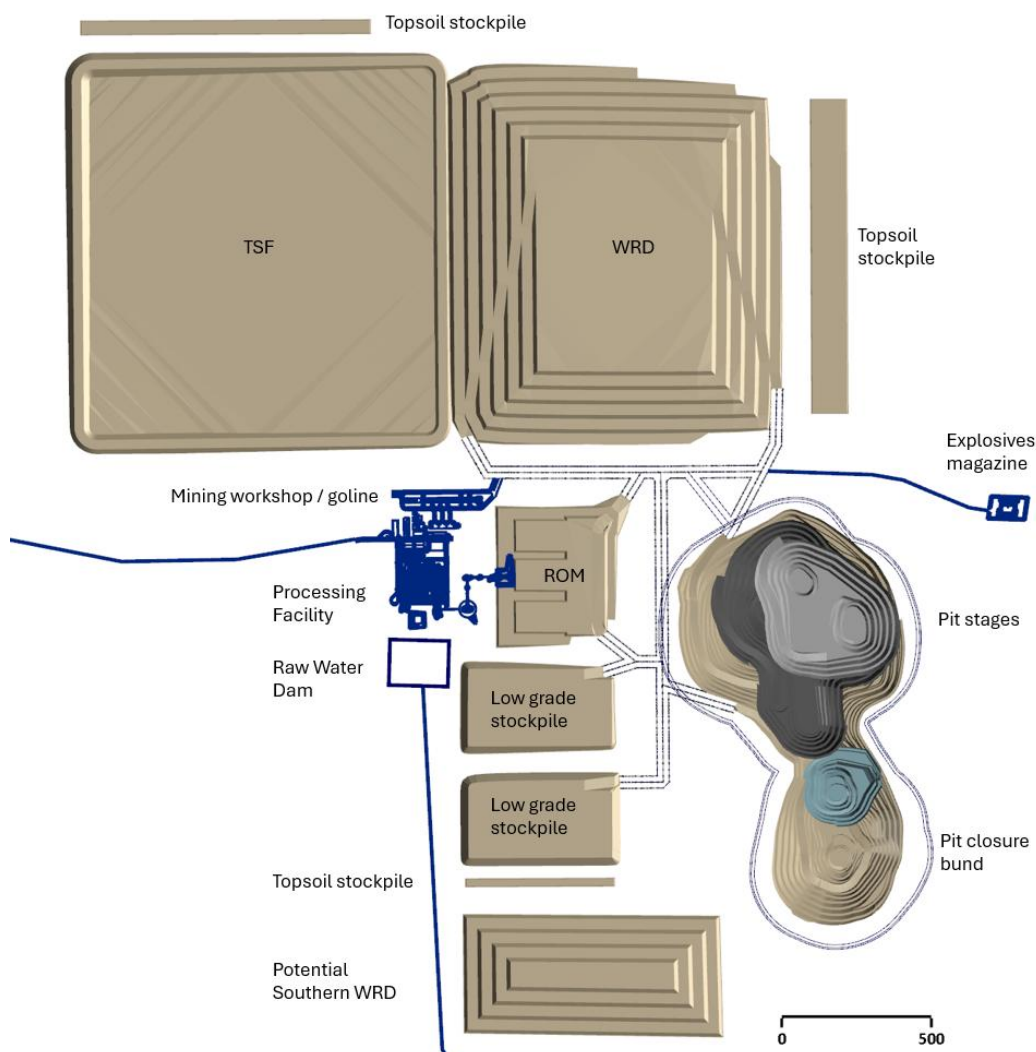
Figure 5.12 High level site layout
