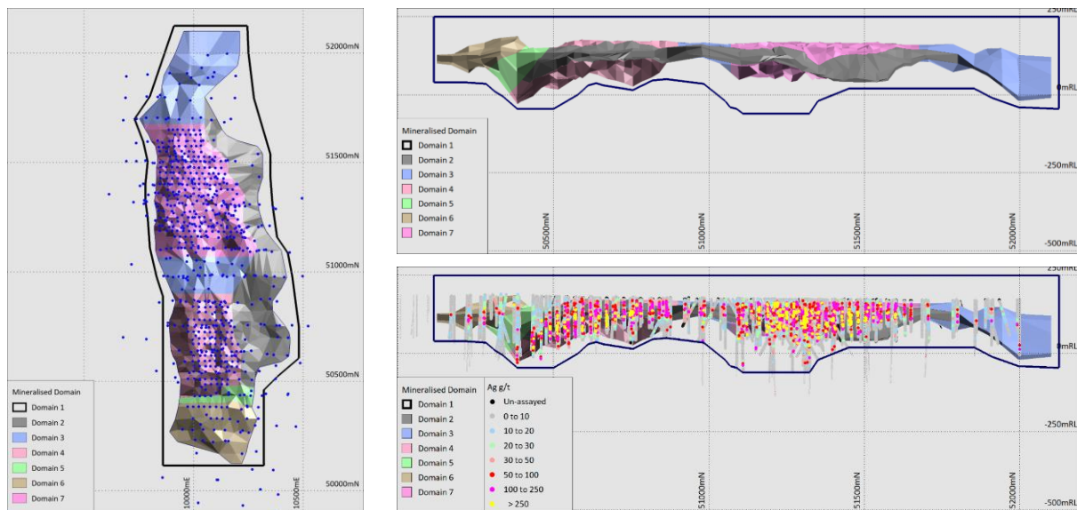
Figure 4.3 2023 Paris MRE mineralised domain plan extents and drill collars (LHS) and domain long section and composite silver grades (RHS)
