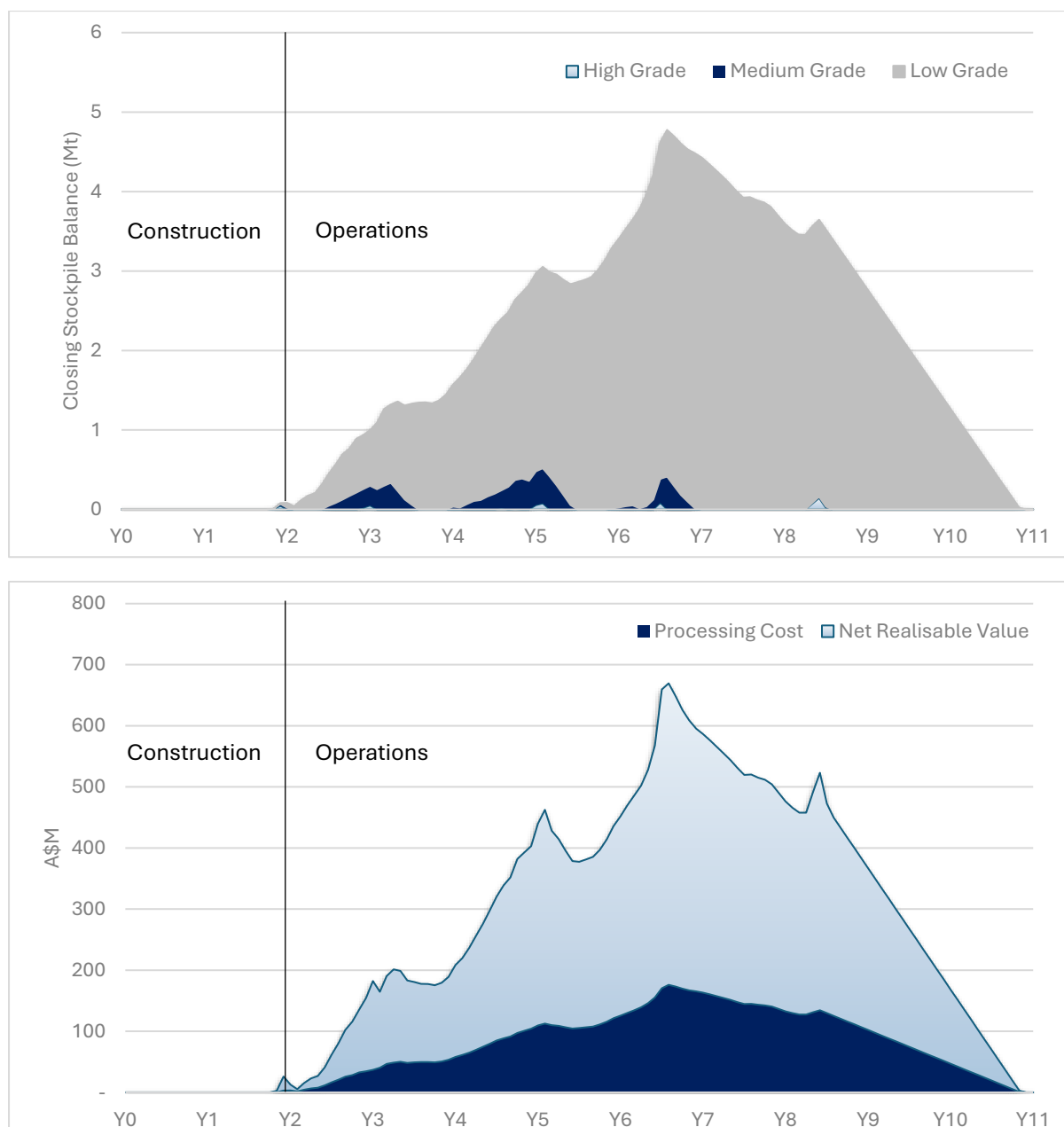
Figure 1.6 Stockpile Balance (top) and Net Realisable Value of Stockpiles (bottom)
