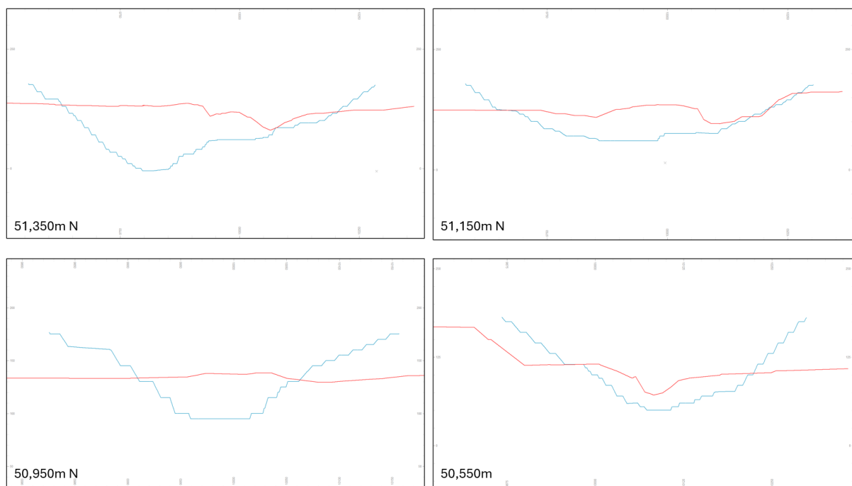
Figure 5.9 Ripability surface (red) and pit design (blue)
