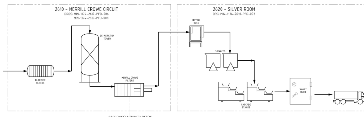
Figure 6.8 Merrill Crowe & Silver Room
