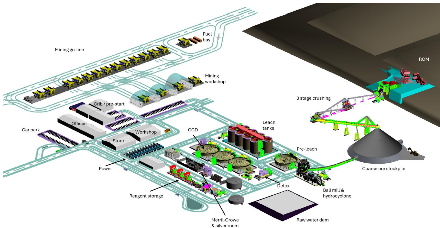
Figure 6.2 General site layout
