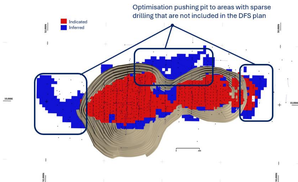
Figure 4.5 Areas of potential for resource growth near Paris
