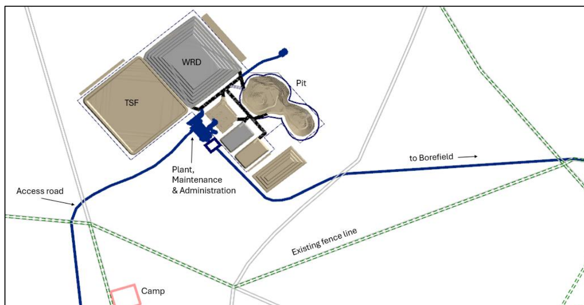
Figure 1.4 Simple flexible site layout on flat ground
