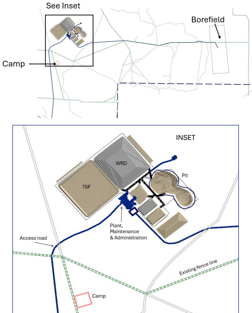
Figure 7.1 Site layout
