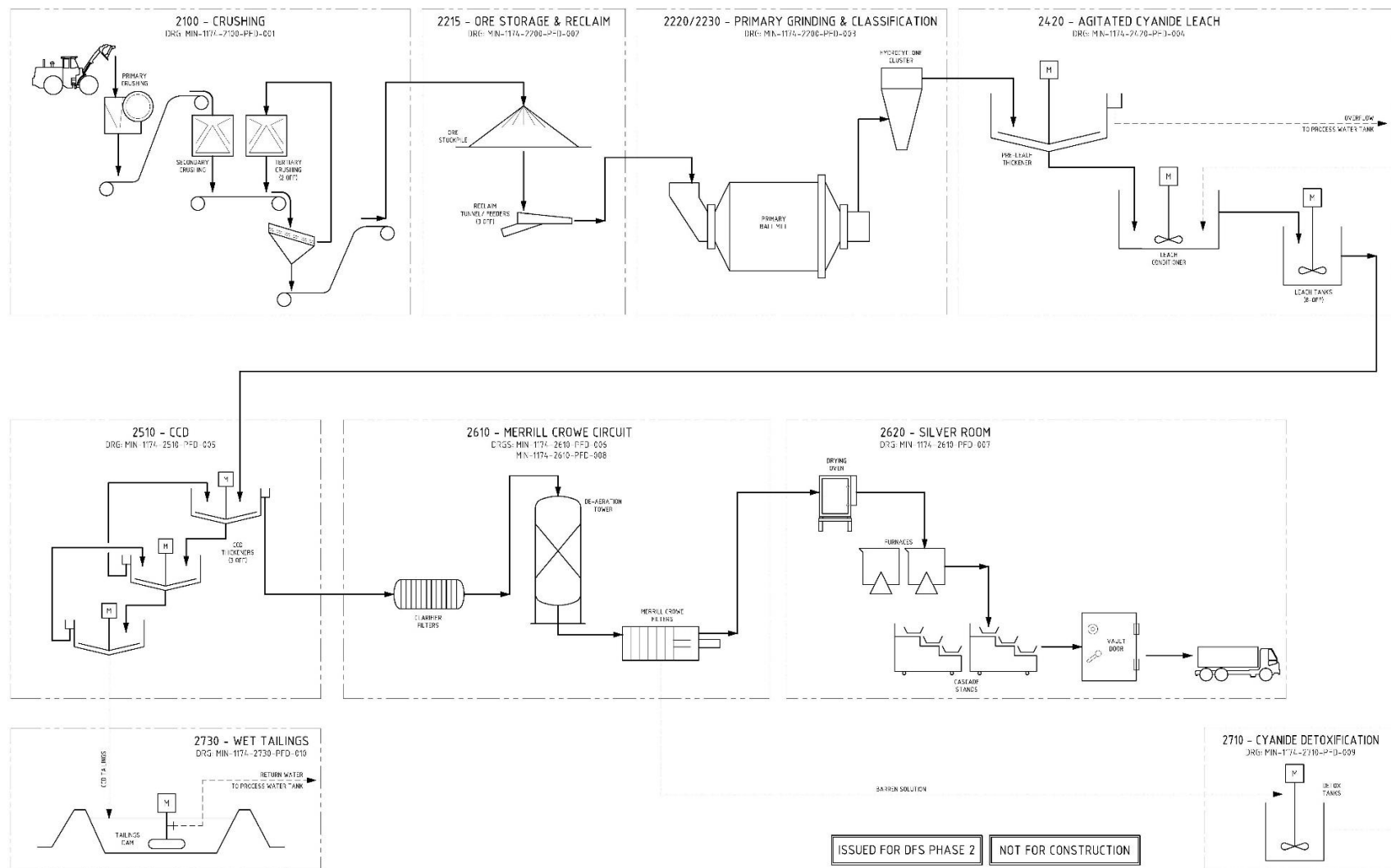
Figure 6.1 Simplified process flowsheet
