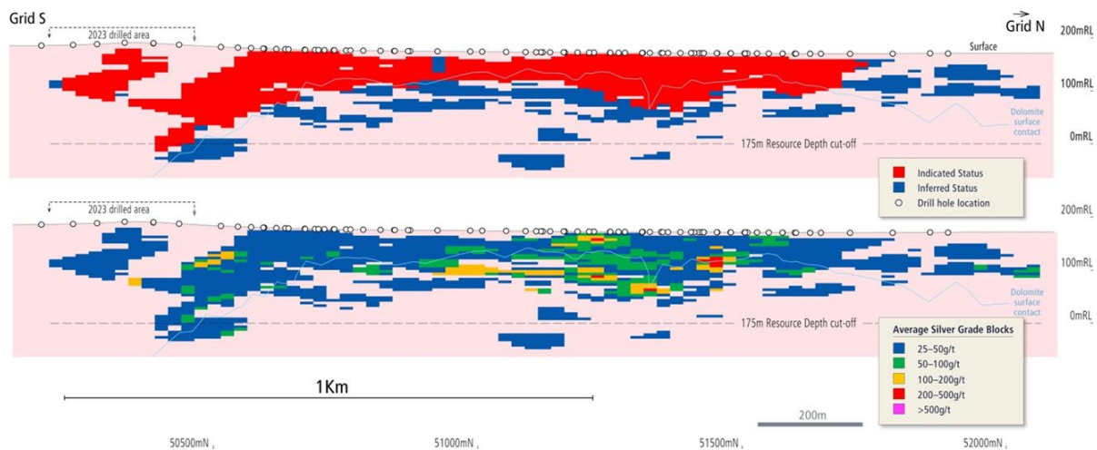
Figure 4.2 2023 Paris MRE long section (10,000mE, +/-25m section) showing distribution of Indicated and Inferred category (top) and average block silver grade (below)
