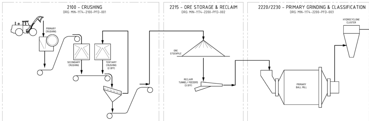
Figure 6.4 Ball Mill Grinding and Hydro-cyclone Classification
