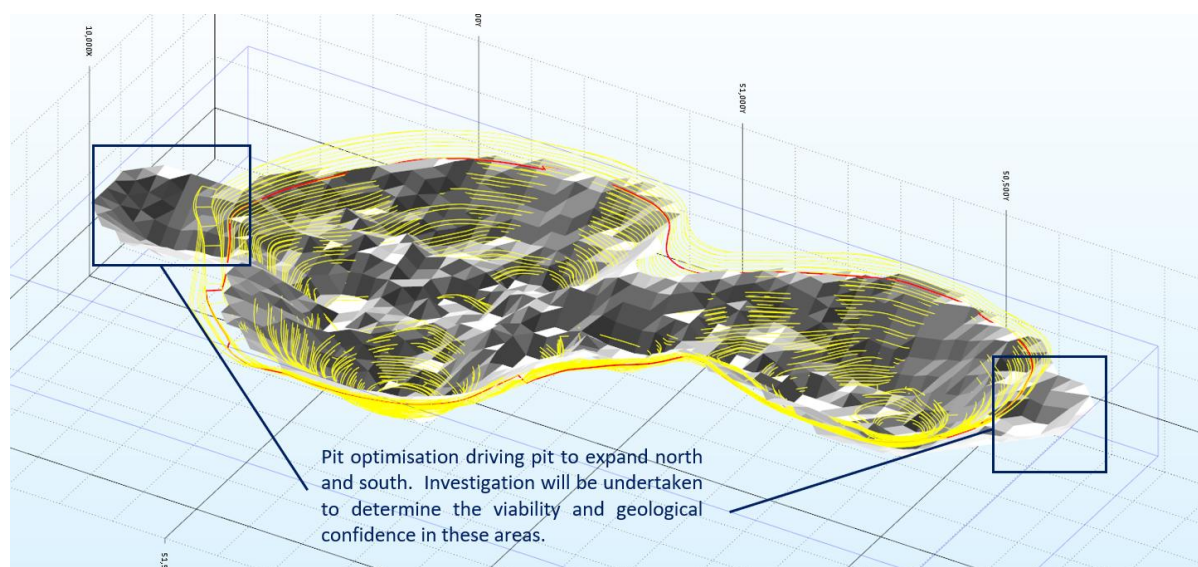
Figure 5.3 Pit Optimisation Pit Shell 26 (grey) compared to DFS pit design (yellow)
