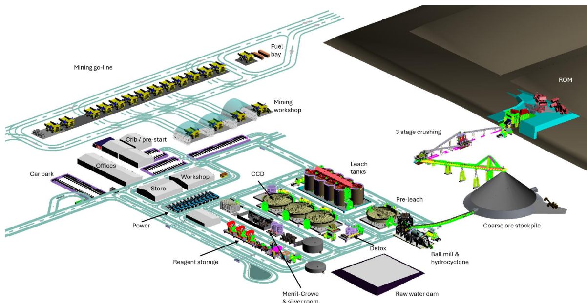
Figure 1.7 Conventional process: crush–grind–leach–Merrill–Crowe silver recovery
