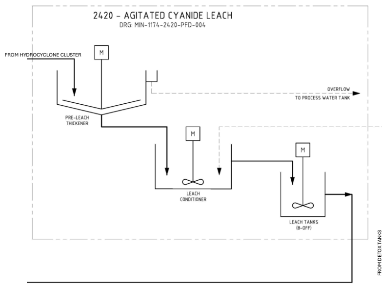
Figure 6.6 Leaching circuit
