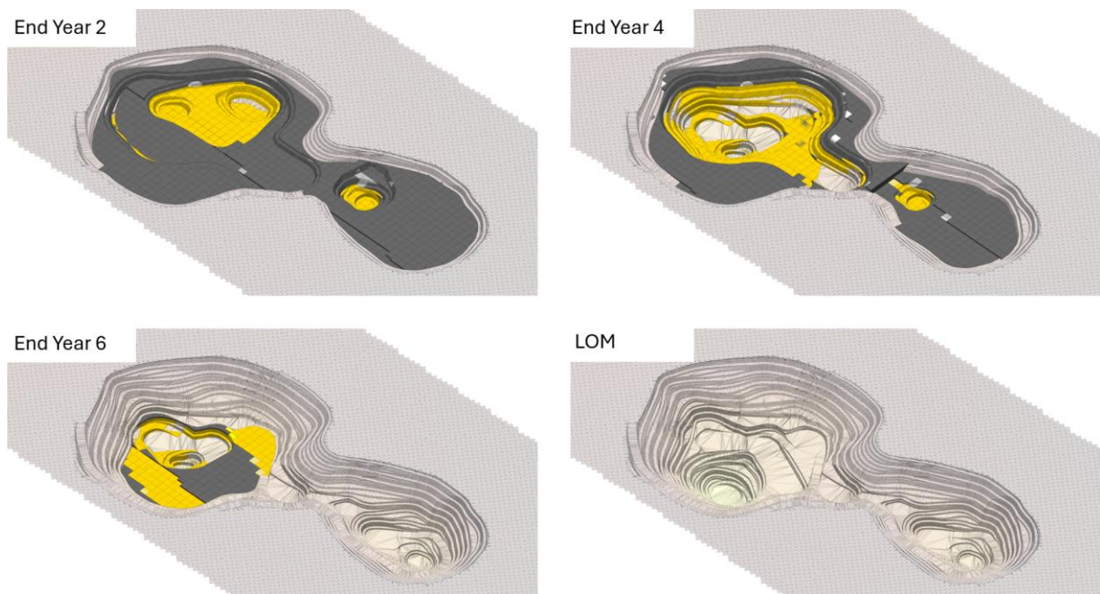
Figure 5.5 Face positions of the pit over the mine life
