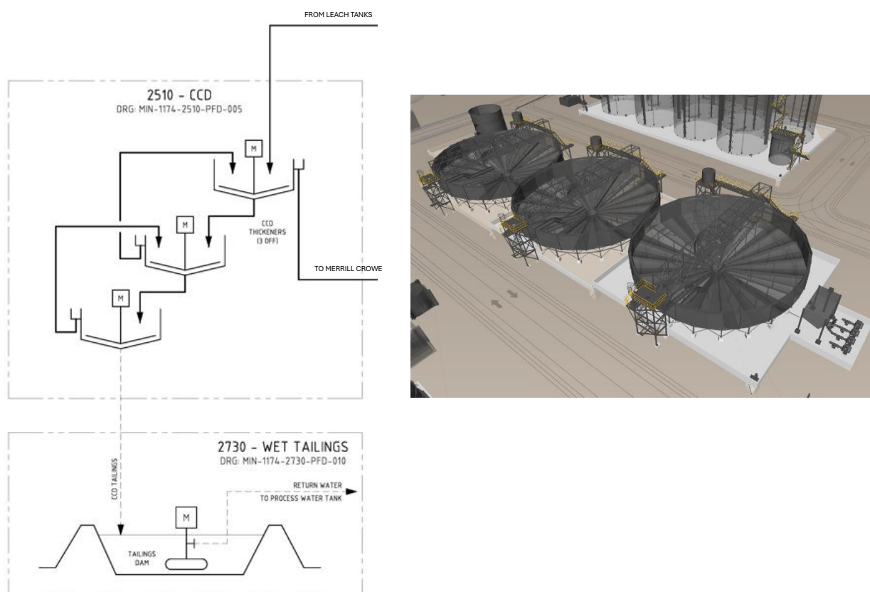
Figure 6.7 Counter-Current Decantation – flow diagram (LHS) and model (RHS)
