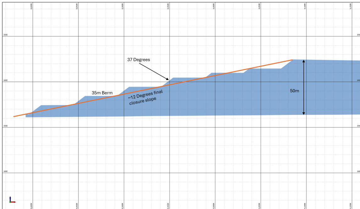
Figure 5.10 Cross section of dump as built (blue) and closure (orange)
