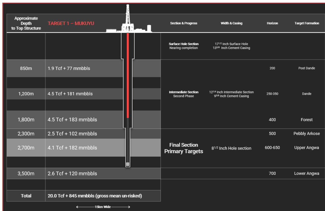
Figure 1 - Illustration of Mukuyu-1 well design.
