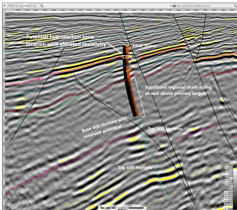
Figure 2 - Mukuyu-1 Preliminary well projection with Gamma Ray log track and location of 200 Horizon intersection near fault.
