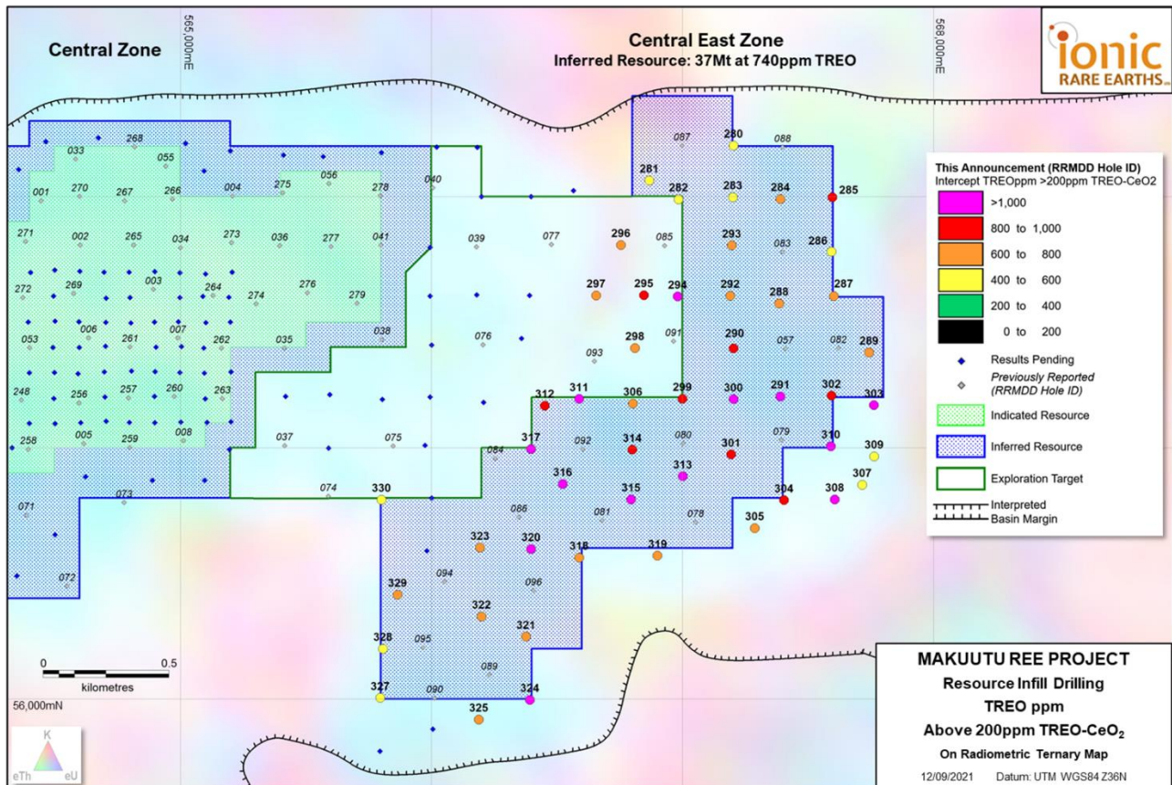
Figure 2: Makuutu Central Zone East drill plan with 50 infill drill holes showing hole locations by drill intercept TREO grade and RRMDD drill hole ID
