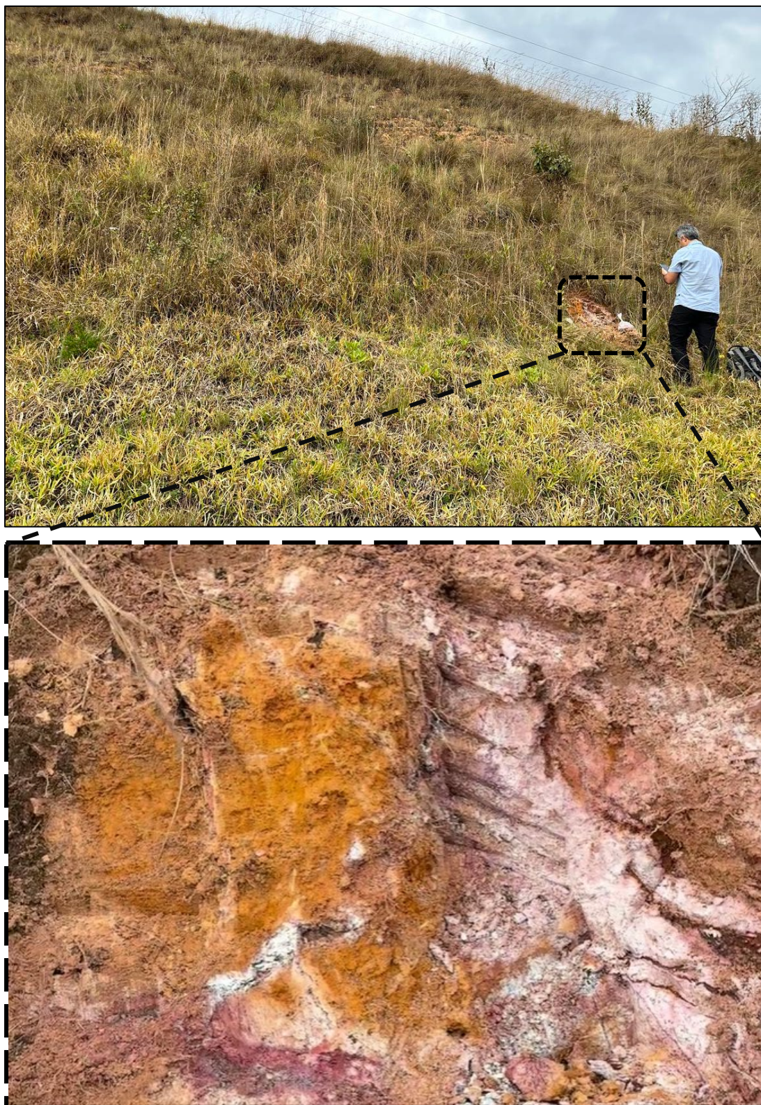
Figure 7: Large saprolite body (top image) with kaolinite/clay outcropping (bottom image) under 0.5 m of overburden at Colossus Project
