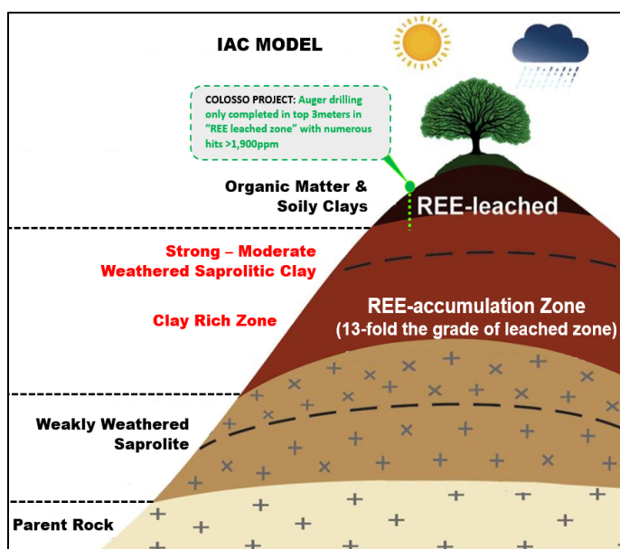
Figure 3: Deposition Model of Malaysian Ionic Clay Project superposition of Colossus Project Auger Drill depths to date 4 .
