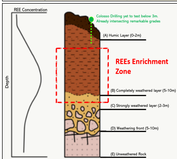
Figure 4: Deposition Model of South China Ionic Clay cross section with superposition of Colossus Project Auger Drill depths to date 6 .
