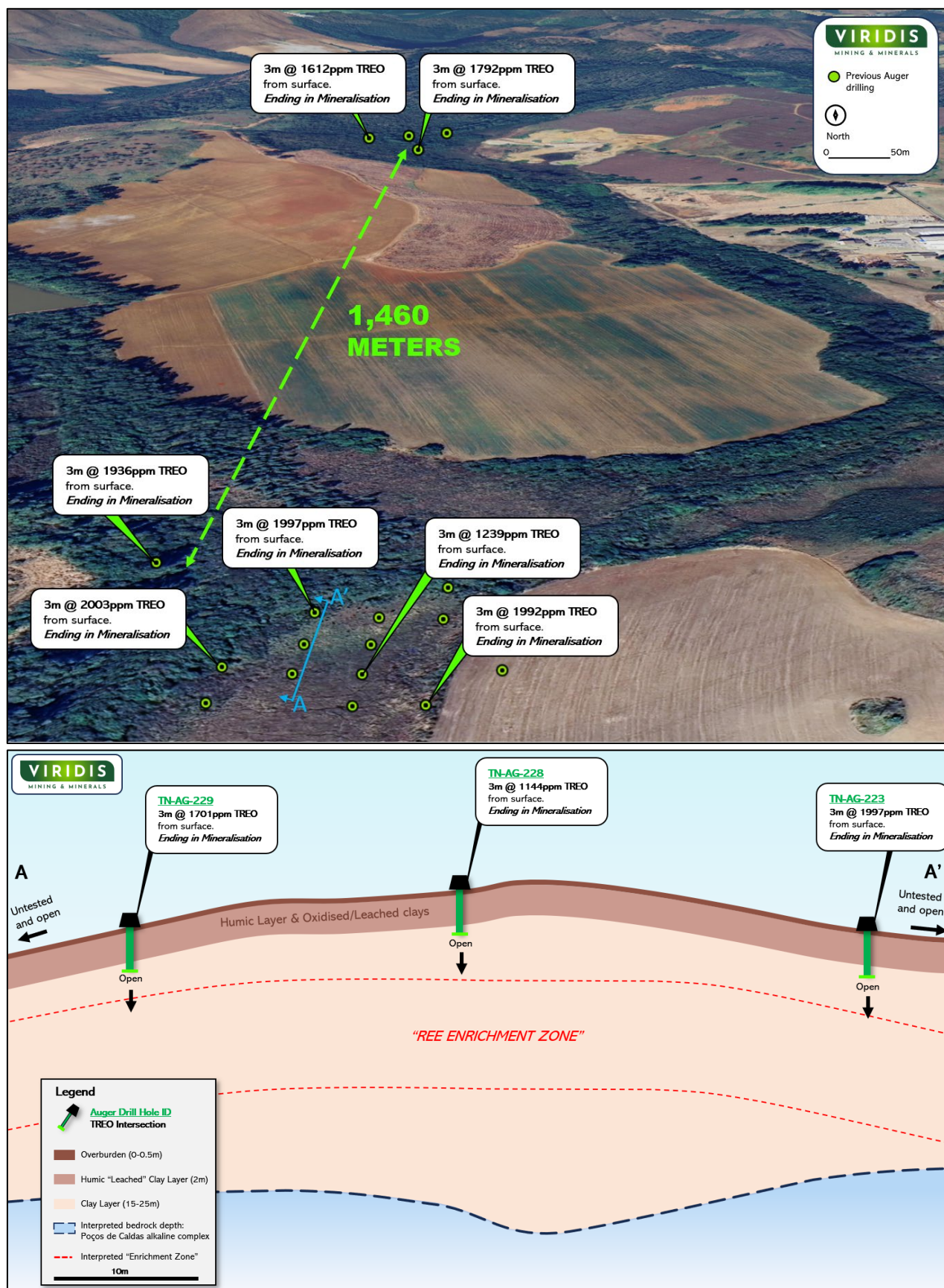
Figure 2: Landscape view of Mining License 009.031/1966 and Exploration License 830.927/2016 (top) and Geologist interpretation of Cross Section AA' looking East (bottom).
