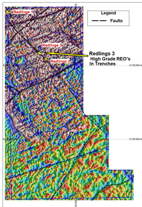
Figure 3 – Jungle Well Structural Interpretation from Magnetic Survey (RTP 1VD)
