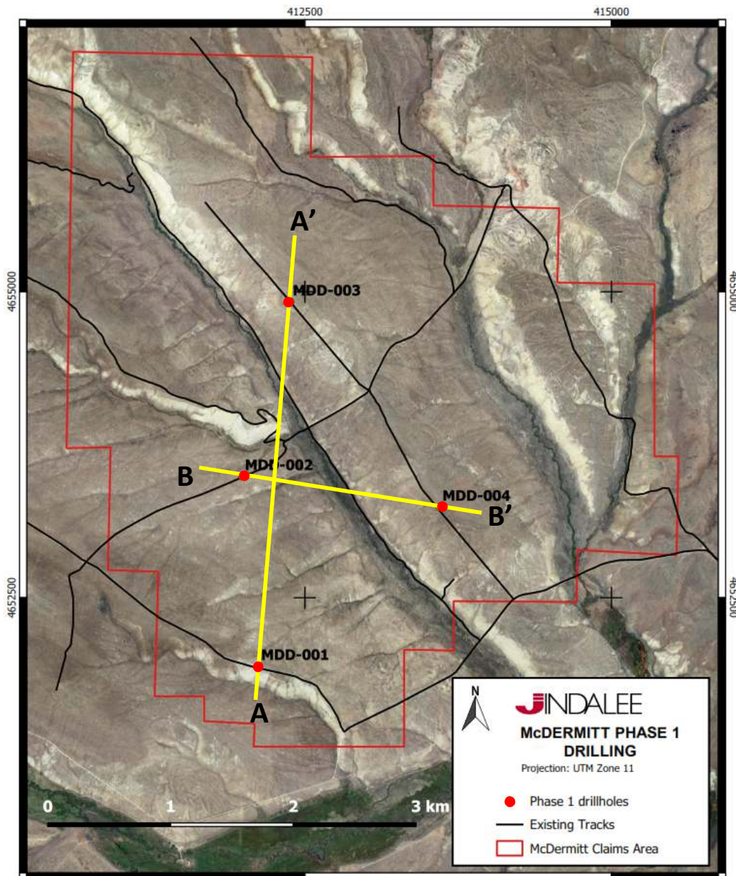
Figure 3 – Recent drill holes at McDermitt, showing the locations of cross-sections A-A', and B-B'.
