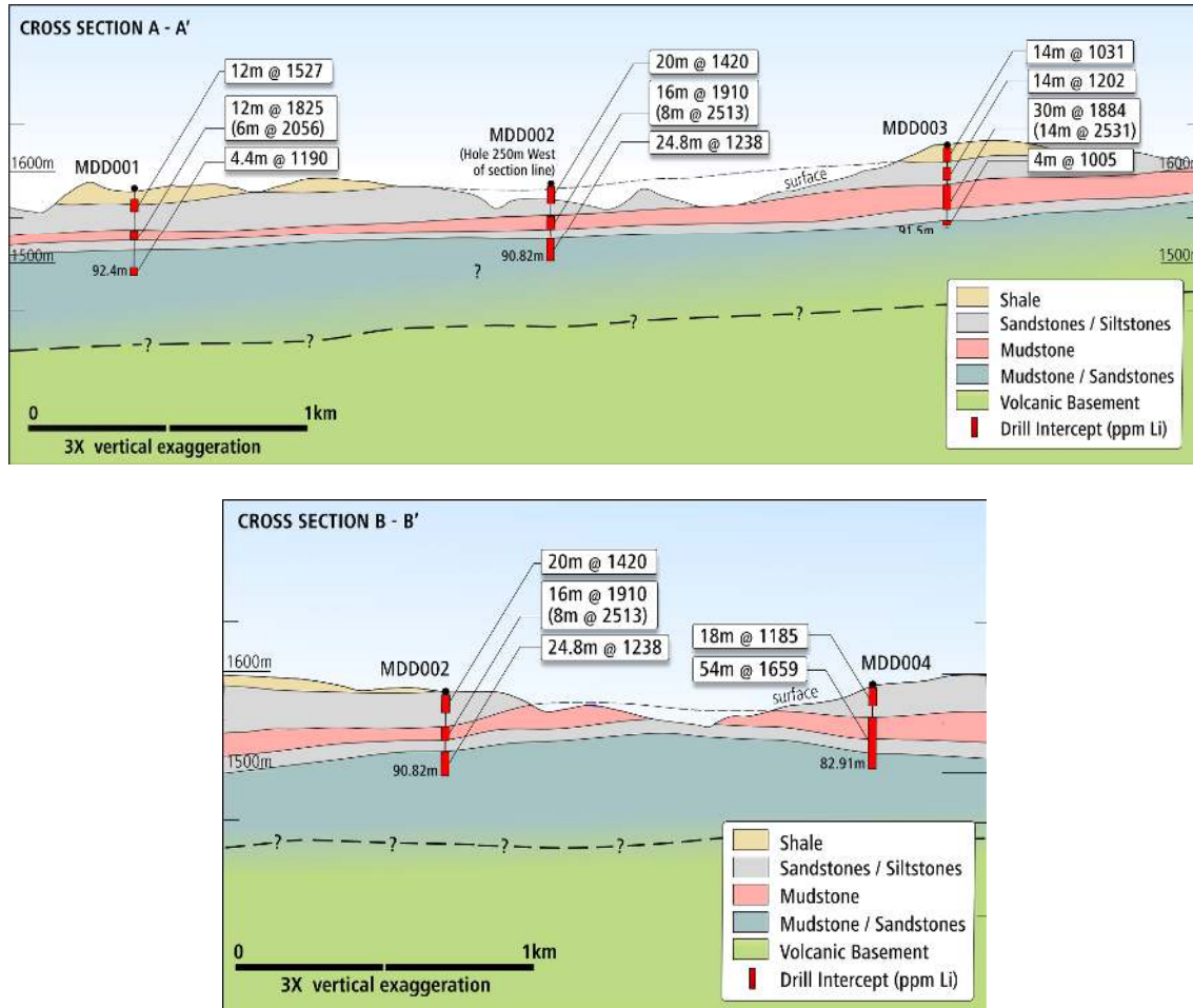
Figure 4 – Schematic cross sections across the McDermitt project, showing significant intercepts and interpreted geology.
