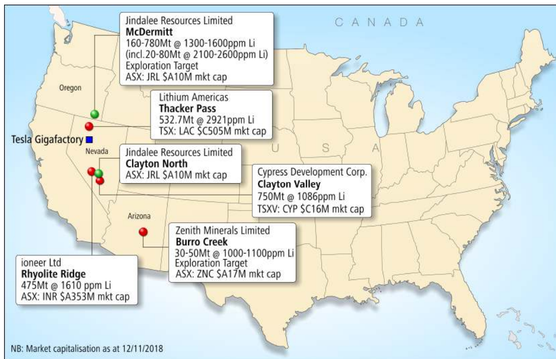
Figure 6 – Location of the sediment hosted lithium projects listed in Table 2.
