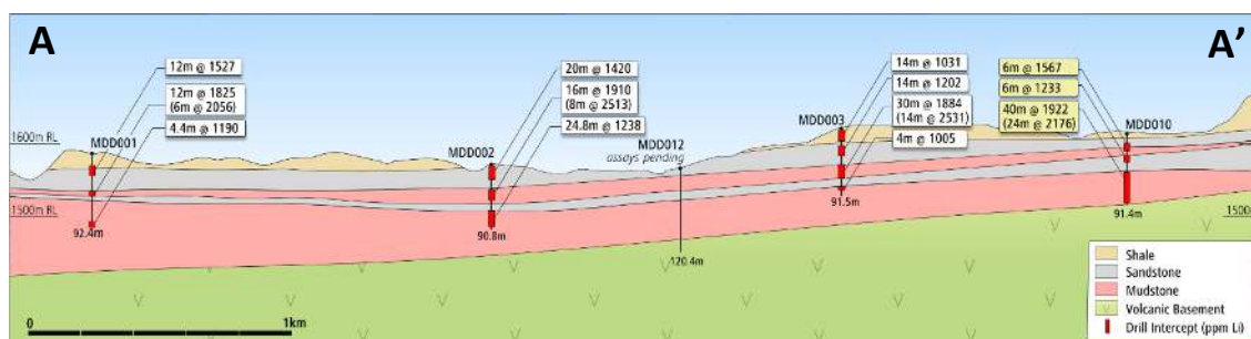
Figure 2 - Cross-section (schematic; vertical exaggeration ~3:1) showing significant intercepts from the 2018 and 2019 drill programs. NB: assays for hole MDD-012 are pending.
