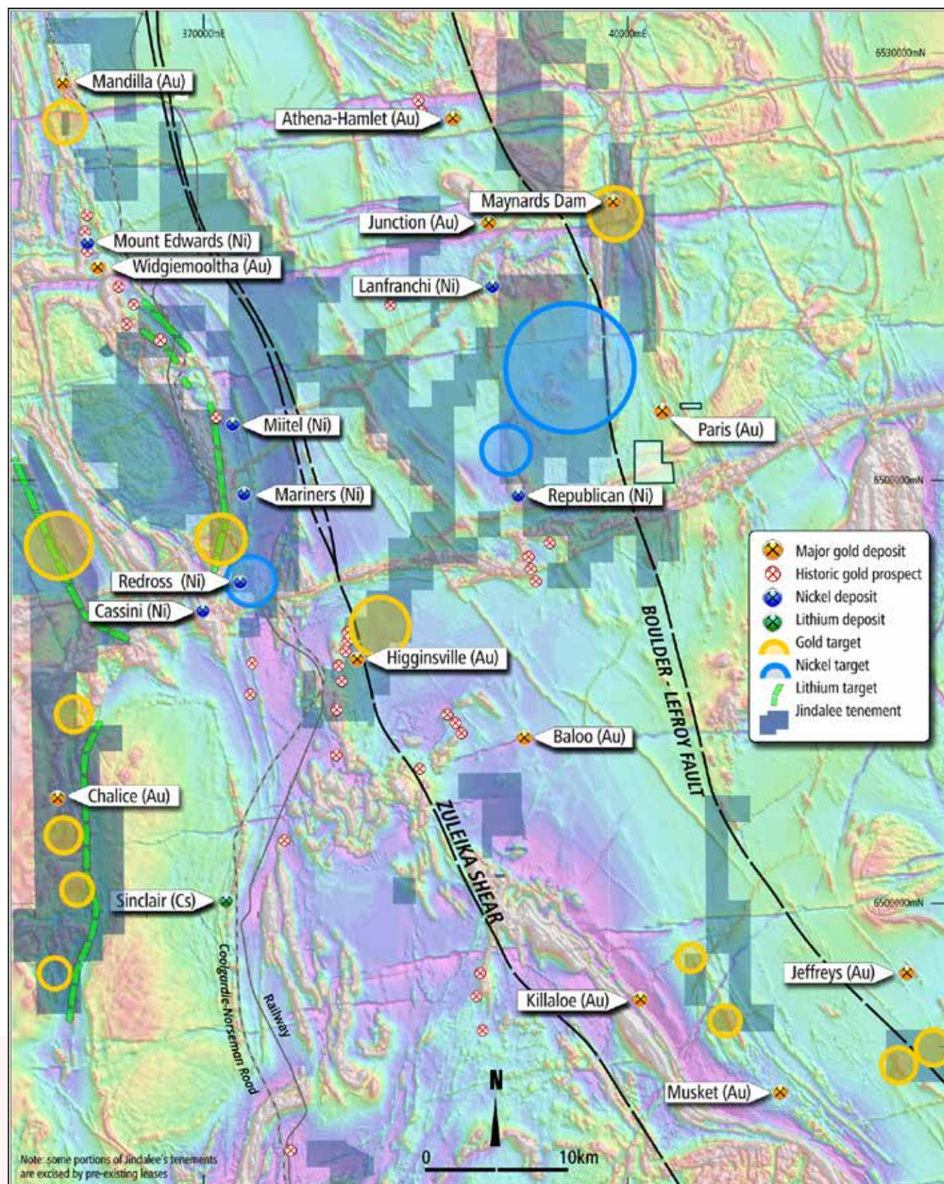
Figure 4. Widgiemooltha Project tenements (at 30 June 2021) over aeromagnetic imagery. Note some portions of the tenements are excised by pre-existing mining and other leases.
