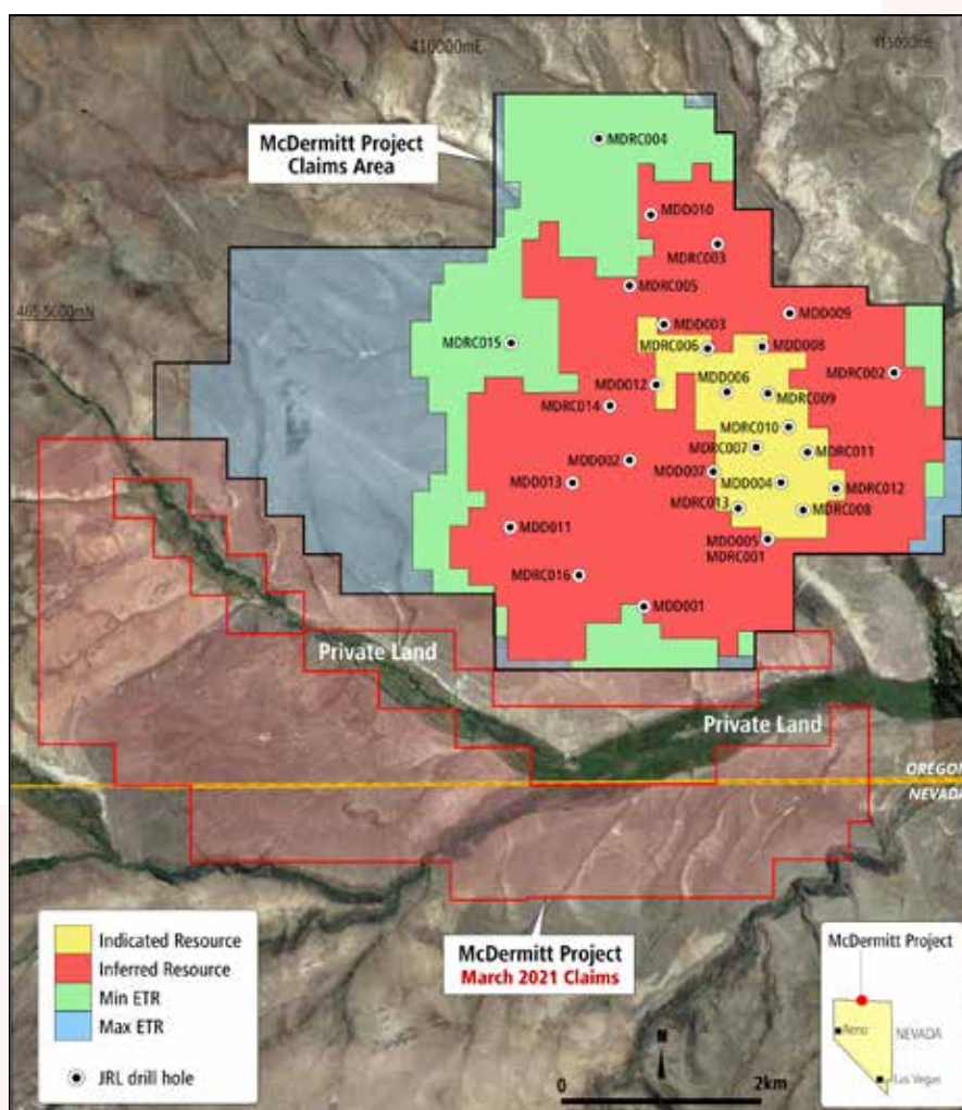
Figure 3. Plan showing McDermitt Resource 1 and Exploration Target 1 Areas & March 2021 Claims.
