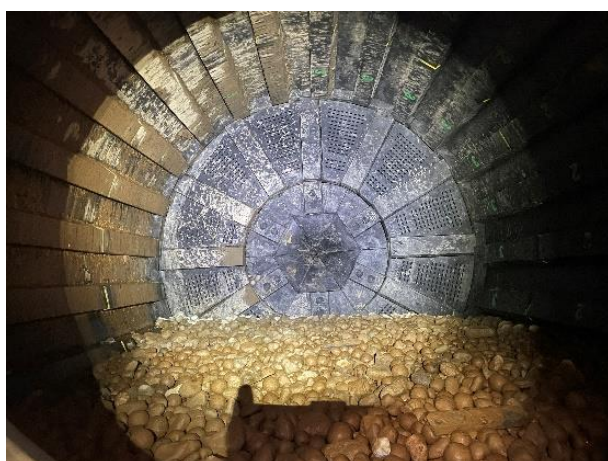
Figure 3. New Mill liners installed
