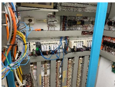
Figure 6. New PLC
