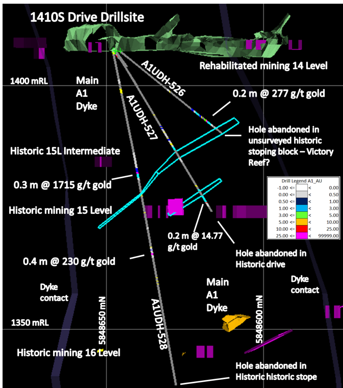
Figure 11: cross section viewed southeast along 230 Mine grid azimuth, illustrates the location of the drillholes A1UDH-526, -527 and -528 drilled from the 1410S Drive, with respect to the A1 Mine workings, reported in this announcement. Modern drives (green) and the interpreted historic workings (magenta), surveyed (amber) and unsurveyed historic stopping (blue).
