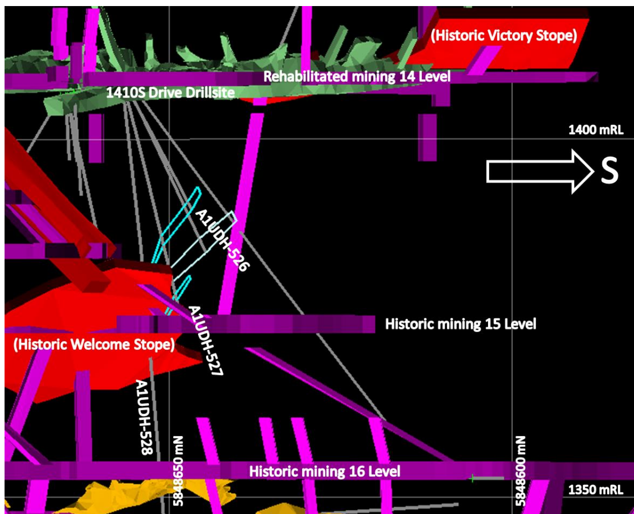
Figure 12: Longitudinal section looking East showing drilling traces (grey), modern drives (green) and the interpreted historic workings (magenta), surveyed historical (amber) and schematic interpretations of historical airleg stoping (red).
