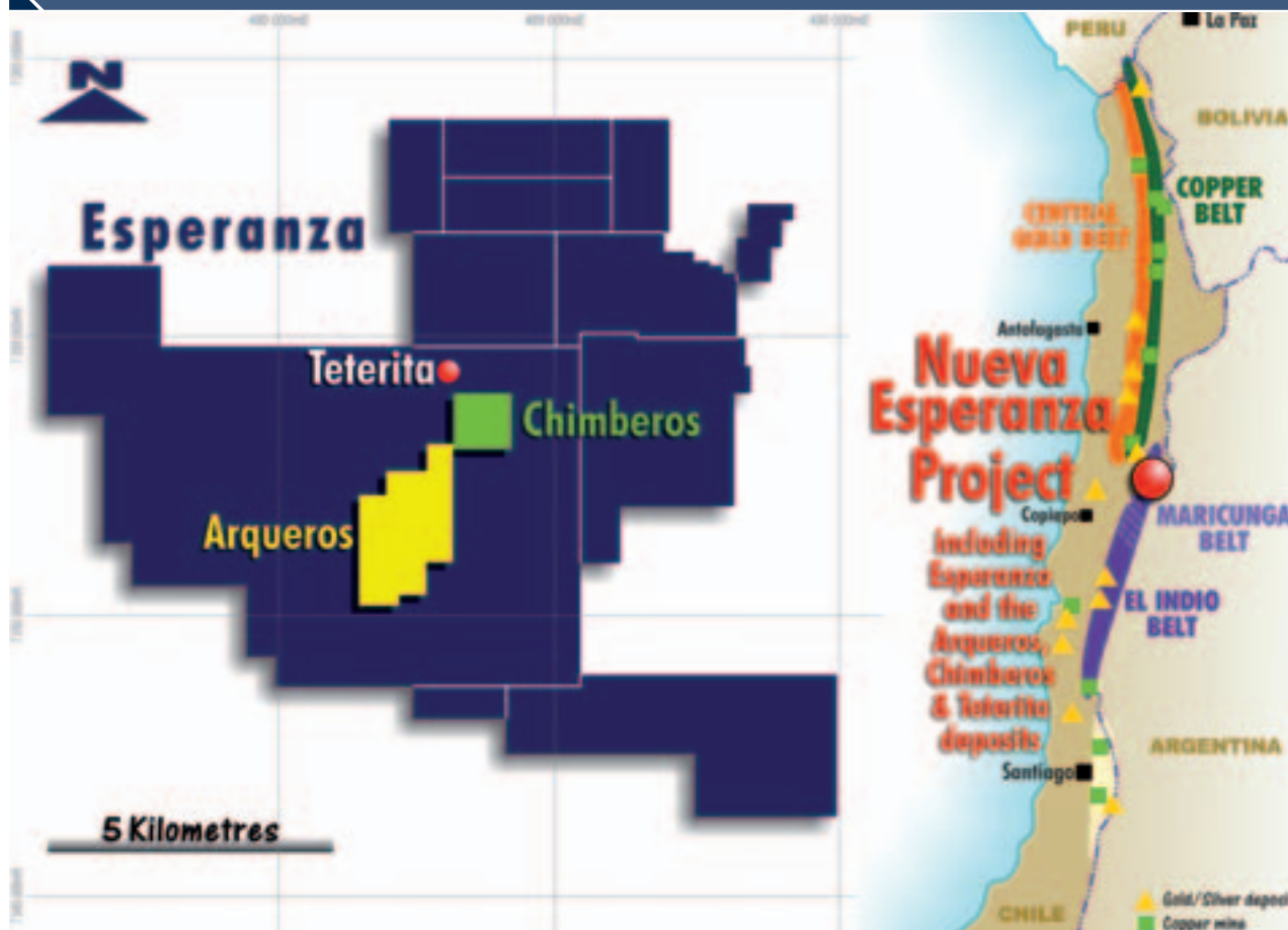
Locations of the Nueva Esperanza Project including the principal deposits Arqueros, Chimberos and Teterita
