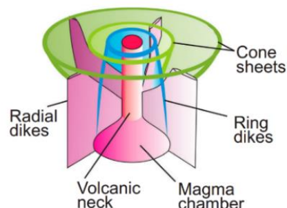
Figure 2: 3D schematic of a carbonatite intrusion*
