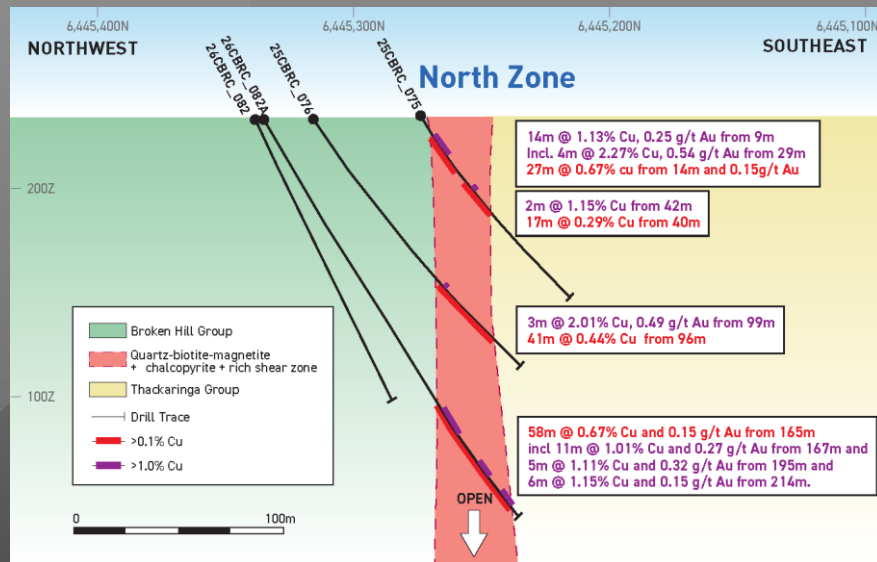
Section B-B'
