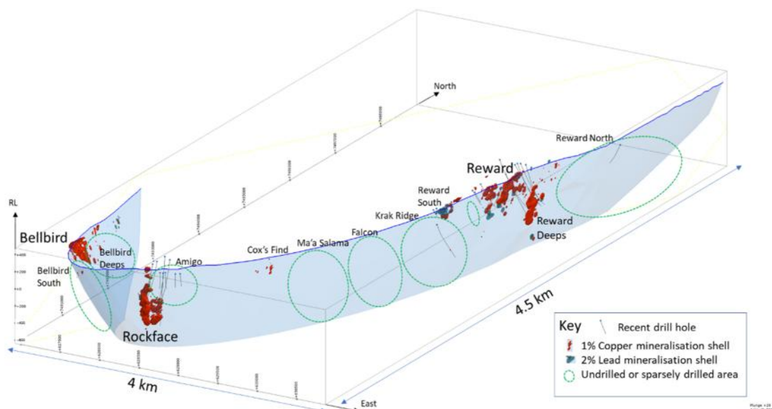
Figure 4: 3D block diagram of the J-fold showing the Jervois mineralisation and current targets.
