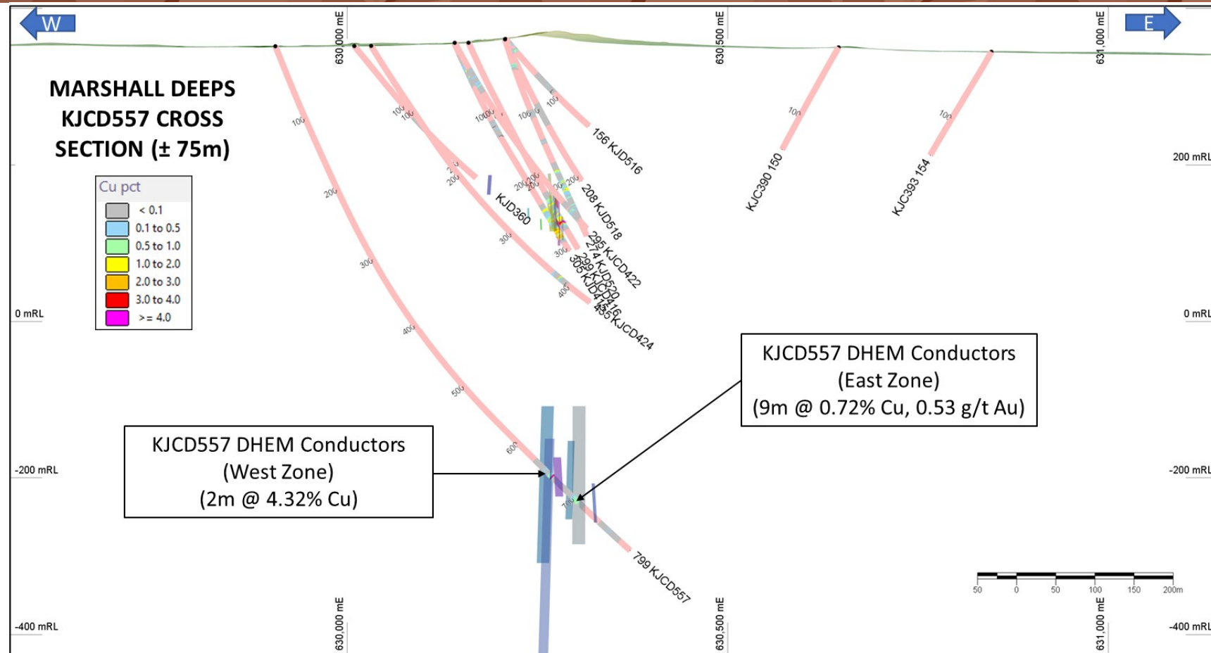
Figure 2: Cross Section through Marshall Deeps hole KJCD557 showing the DHEM conductors associated with both the west and east zones of mineralisation
