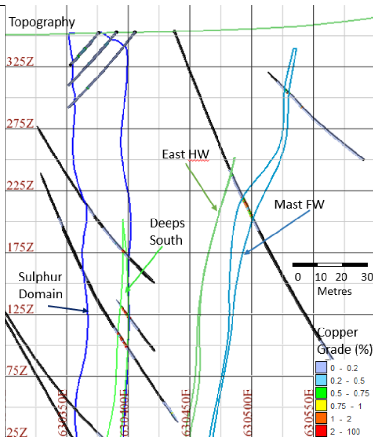
Figure 8. Deeps South and East Lodes, Cross Section (7495350 mN ± 12.5m)
