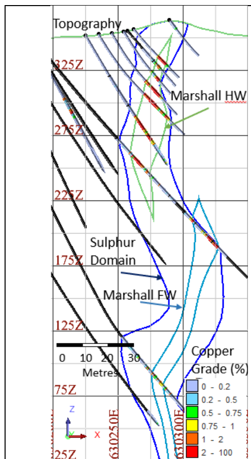
Figure 7. Marshall Lode Cross Section (7494525 mN ± 12.5m)
