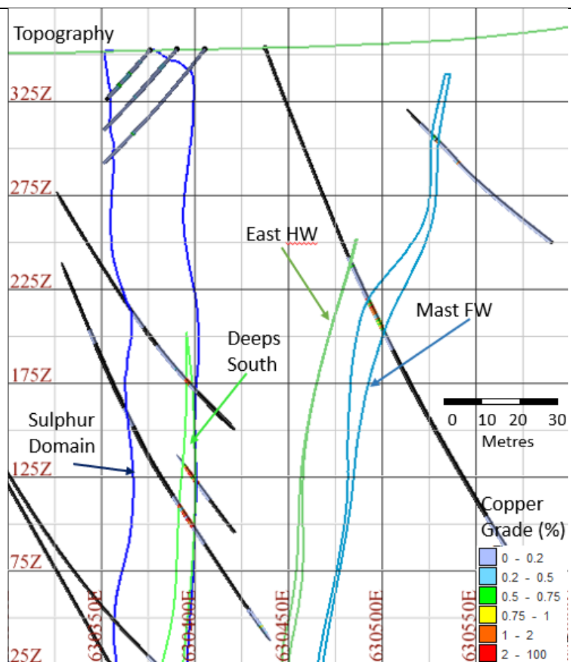
Figure 1-5. Deeps South and East Lodes, Cross Section (7495350 mN \pm 12.5 m)
