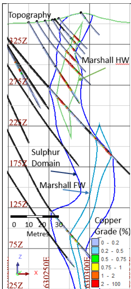
Figure 1-4. Marshall Lode Cross Section (7494525 mN \pm 12.5 m)
