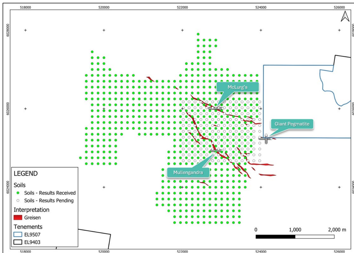
Figure 4: Soil sampling status at Sweetwater
