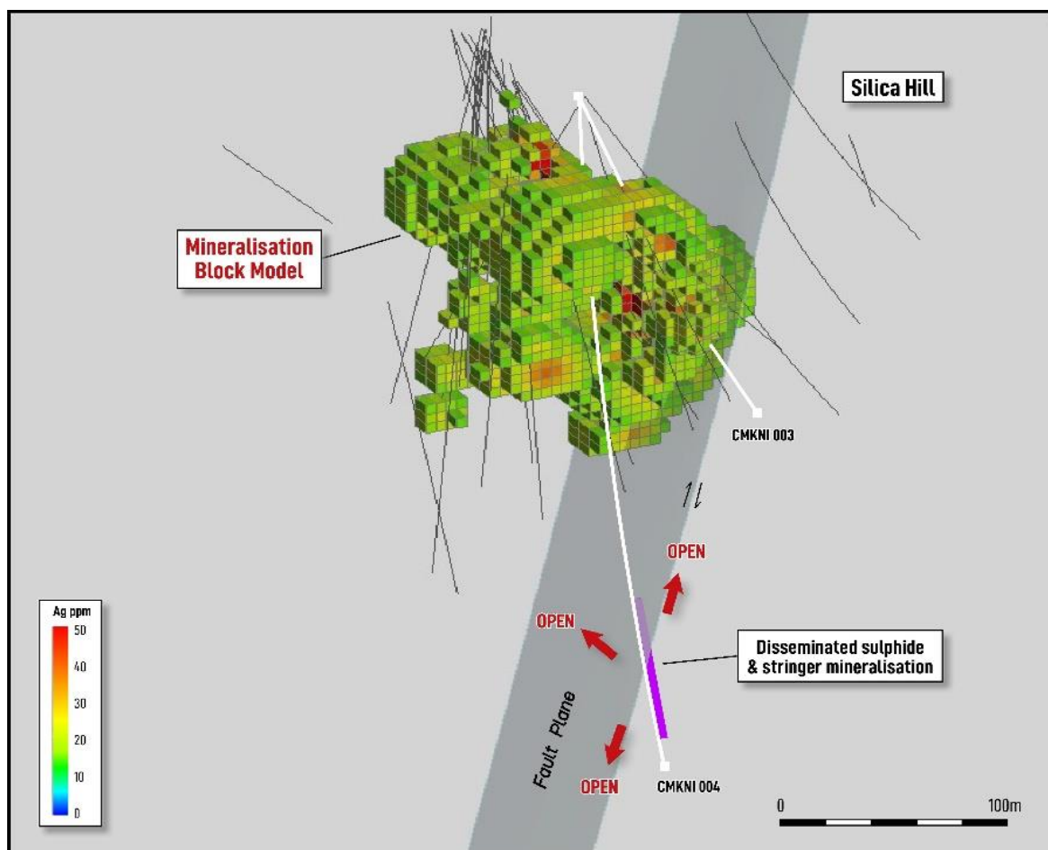
Figure 5: Leapfrog cross-section view showing the current Silica Hill Block Model and drillhole CMKN004 intersecting a new zoned mineralisation located approximately 100m outside the previously modelled mineralisation wireframe, defining a mineralised zone that remains open up- and down-dip and along strike.
