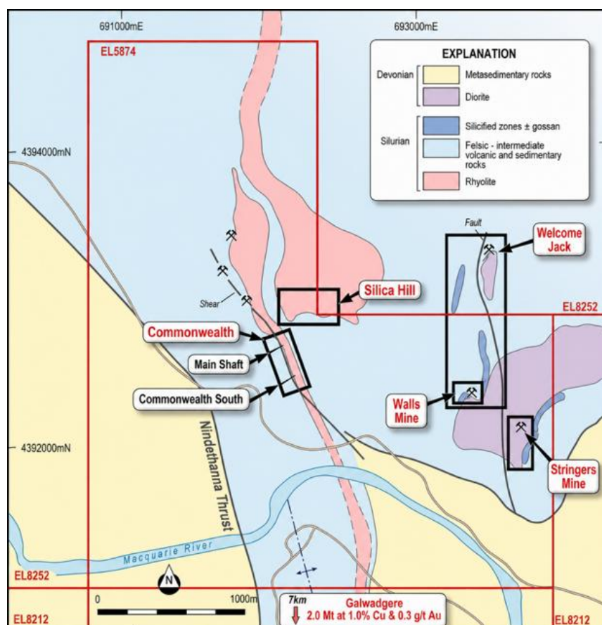
Figure 1: Commonwealth–Silica Hill–Welcome Jack trend highlighting the mineralised corridor, key prospect locations and the geological relationship between Welcome Jack, Walls and Stringers, located in close proximity to the existing Commonwealth–Silica Hill mineralisation.
