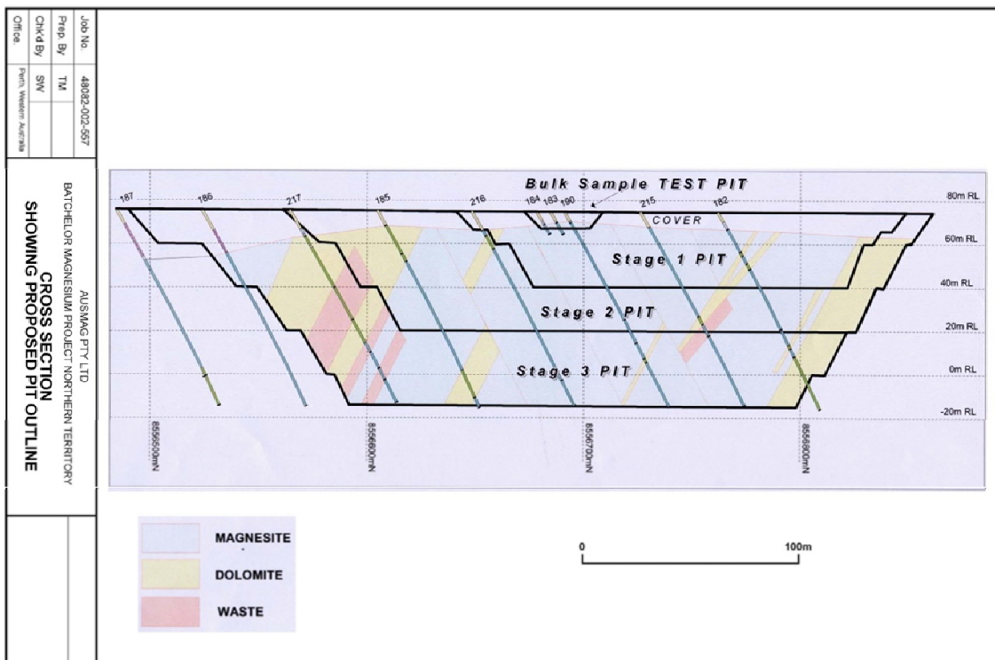
Figure 6 Open pit cross section – staged development variant
