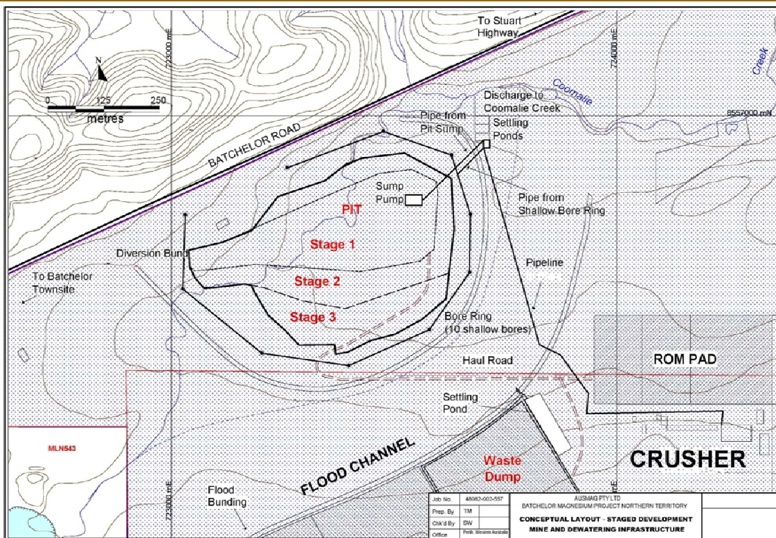
Figure 5 Conceptual layout – staged development variant
