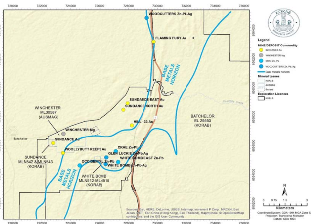
Figure 10 Zinc/base metals horizon at Batchelor
