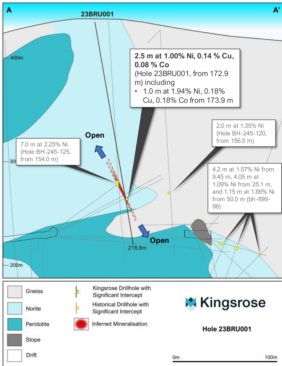
Figure 5: Cross section (Section A-A') showing hole 23BRU001.
