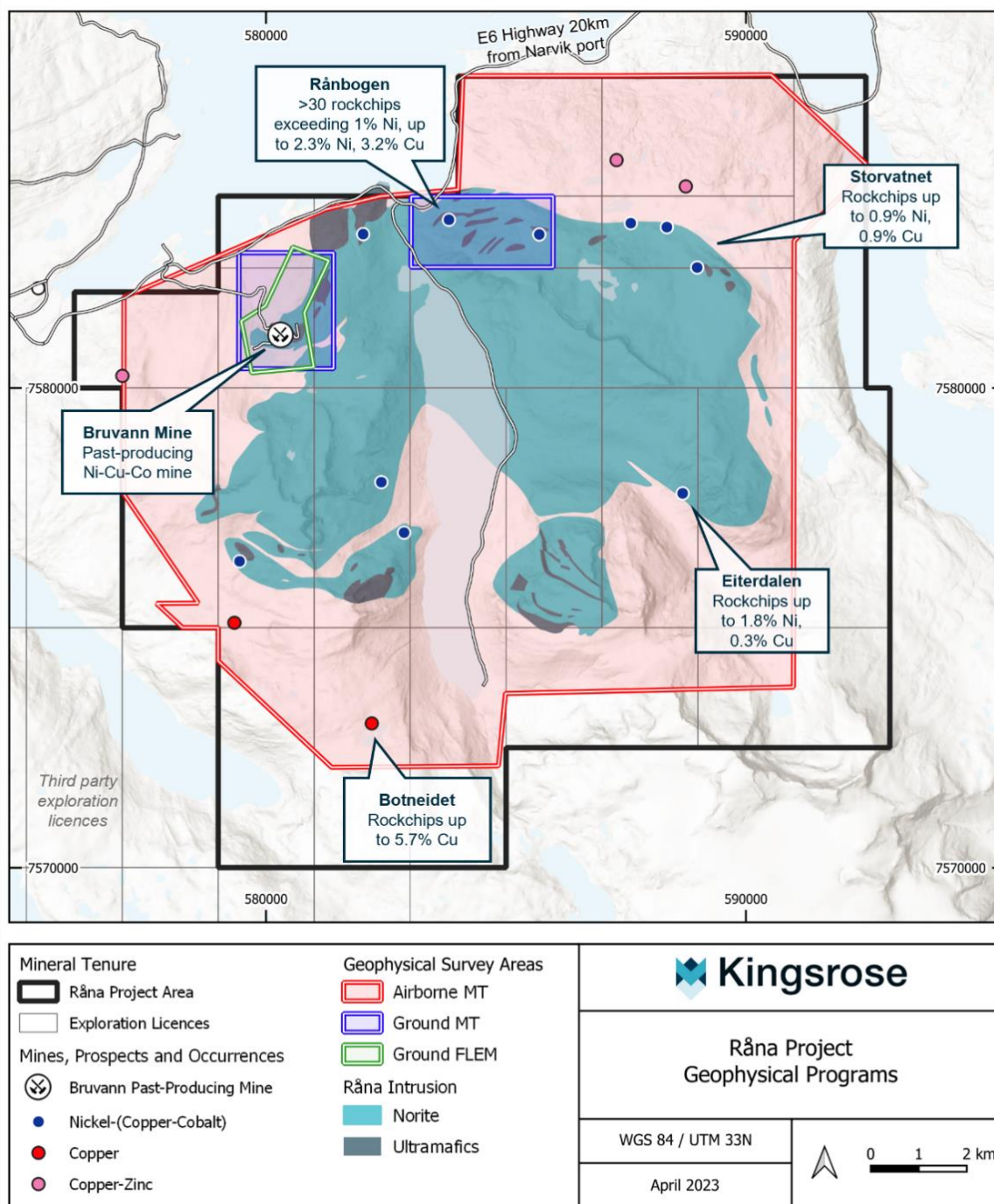
Figure 2: Råna project location, geology, exploration licences and geophysical completed in the quarter.
