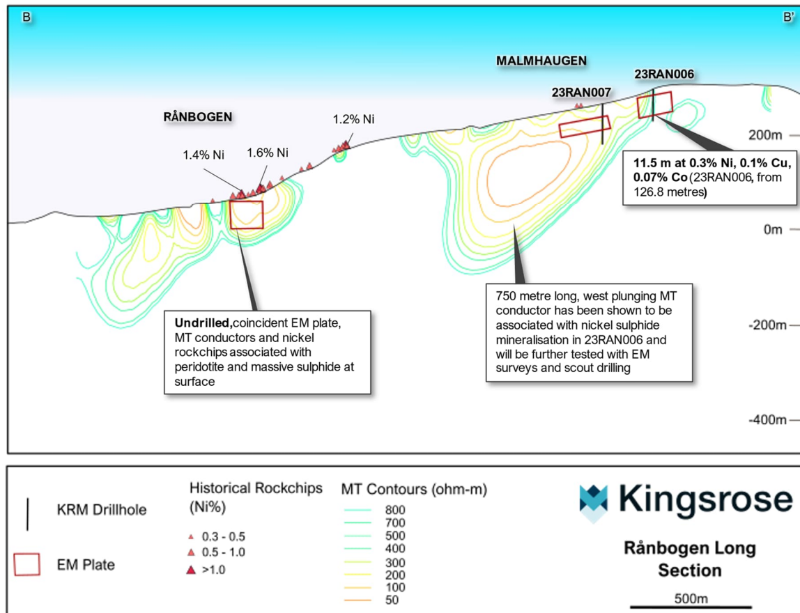
Figure 5: Long section showing highly conductive MT anomalies underlying near surface EM modelled plates and nickel mineralised massive sulphide at surface, Rånbogen and Malmahugen prospects.
