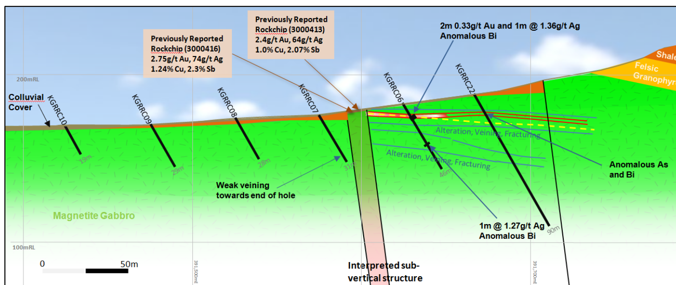
Figure 3: EW cross section along the northern line showing a sub horizontal weakly mineralised structure extending east from the very high grade surface outcrop at the intersection of an inferred vertical structure.
