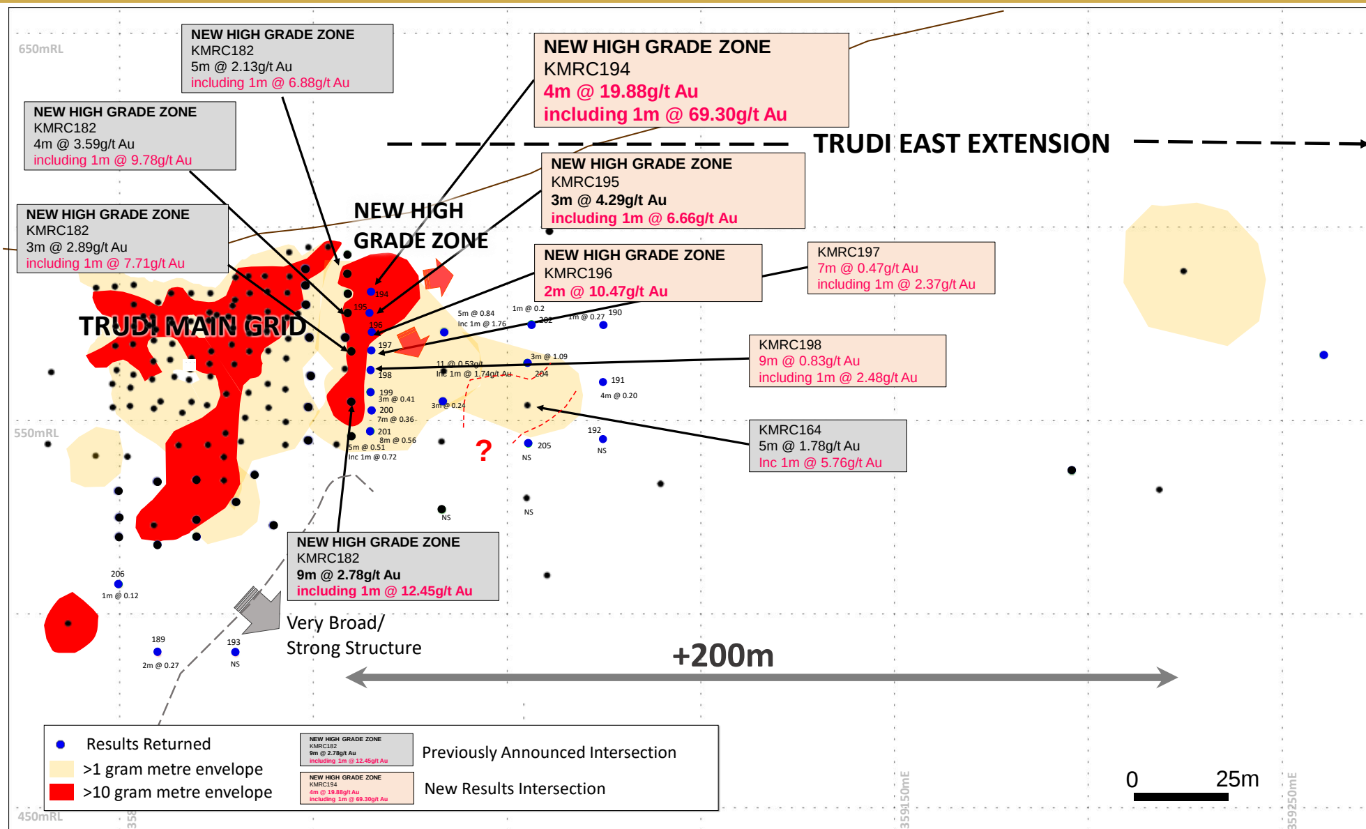
Figure 5: Long Projection of Trudi showing results
