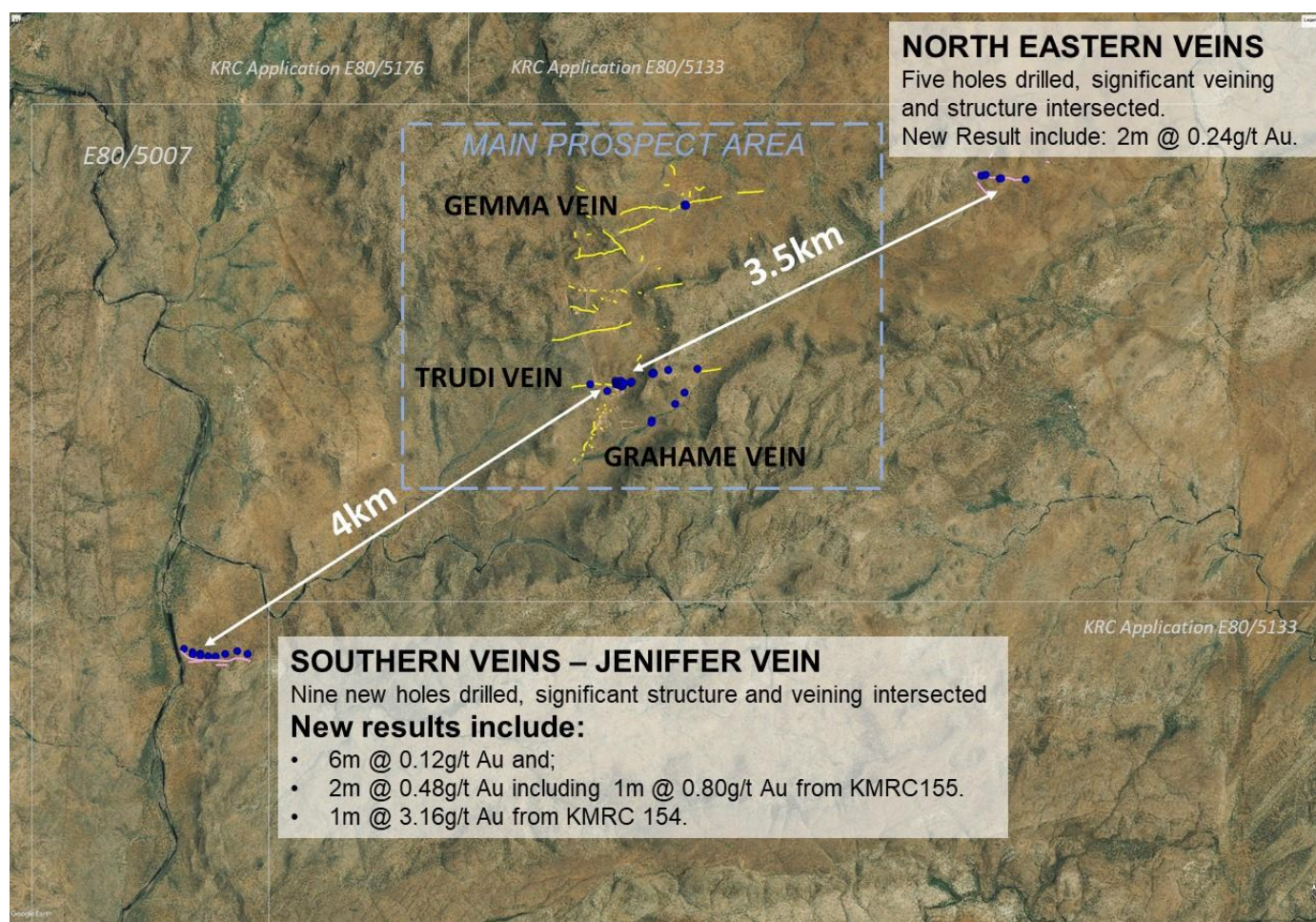
Figure 6: Plan showing location of North Eastern veins and Southern veins in relation to Trudi.
