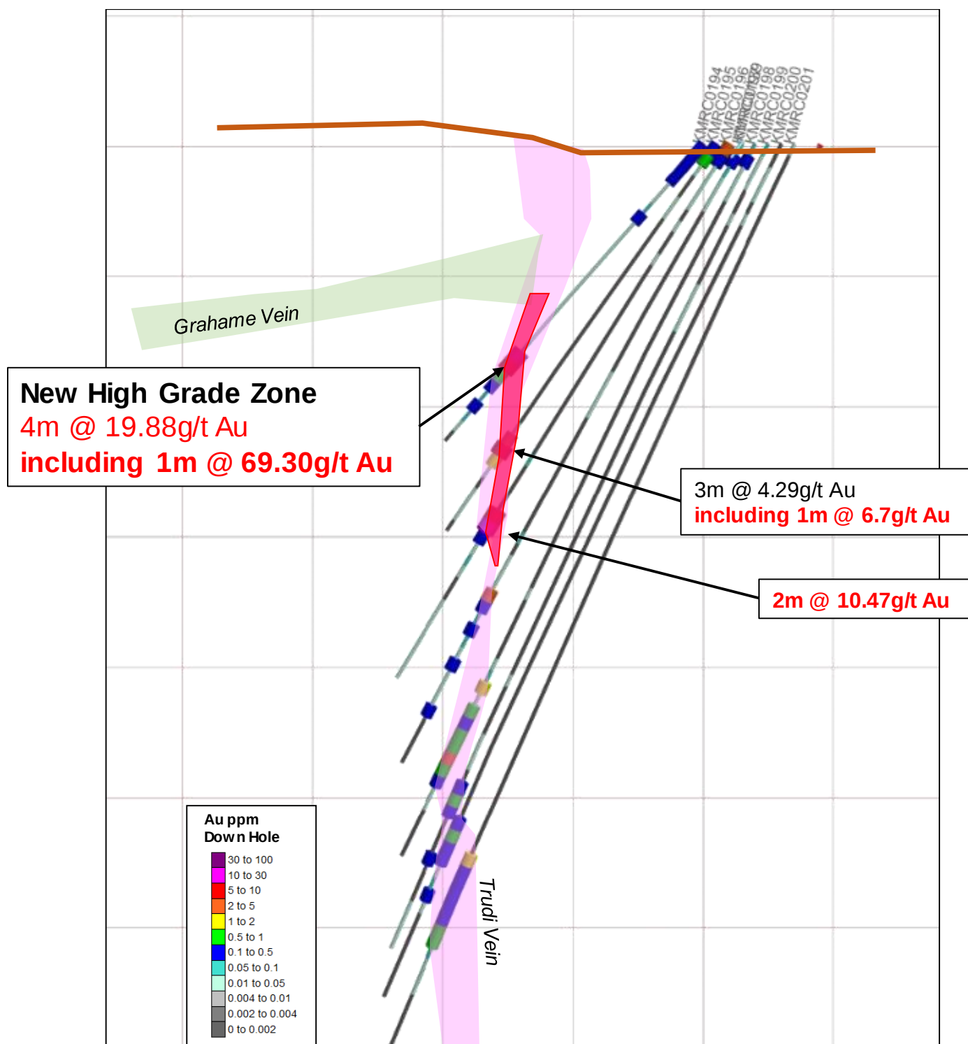
Figure 3 Results and assays pending on 359014mE section looking west
