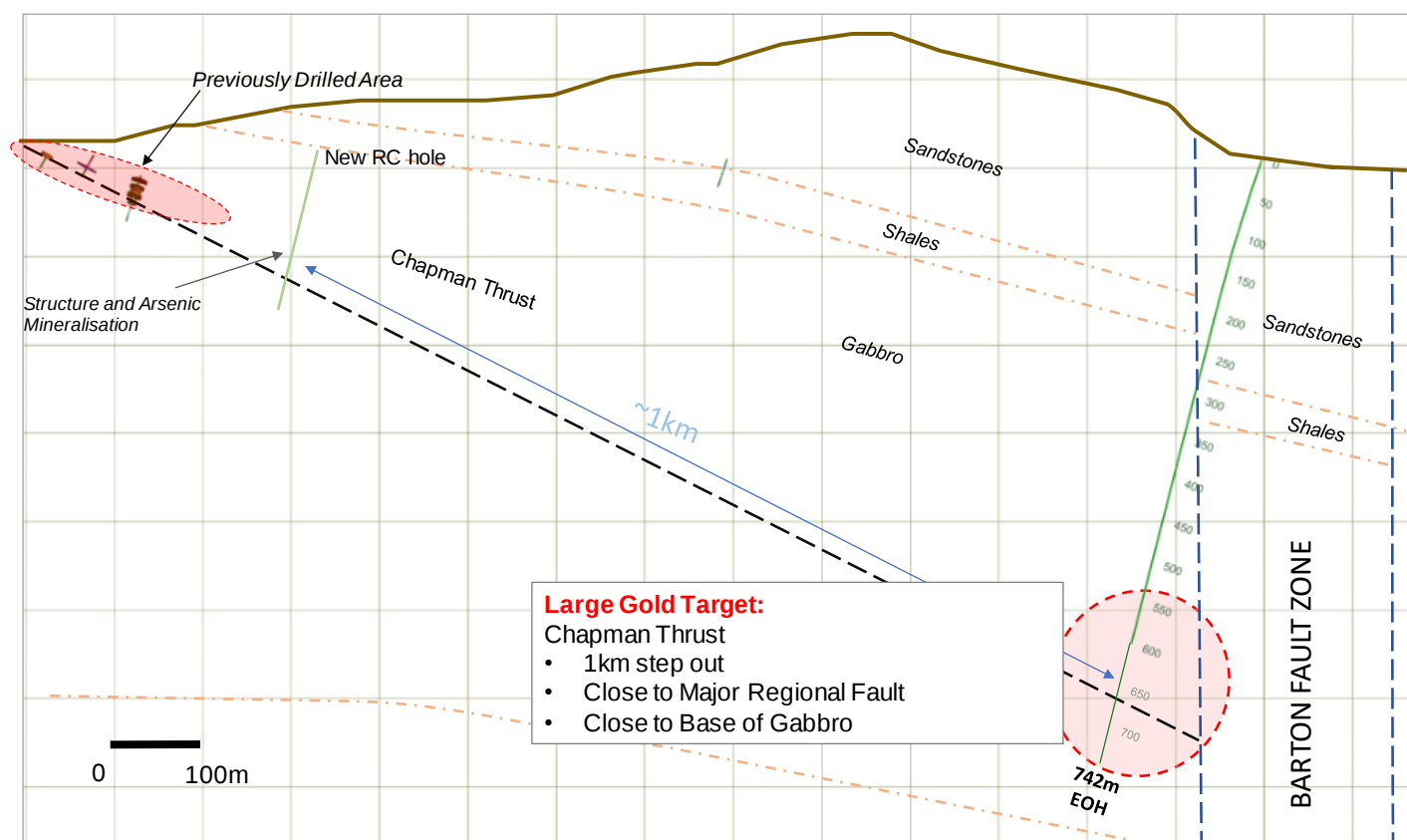
Figure 7 Cross Section of the drill hole, looking South West (235°). Shows interpreted extrapolation of the Chapman Thrust to the target zone close to the Barton Fault. Due to the scale of the section the location of previous drilling, topography and the new RC are diagrammatic (being off section).
