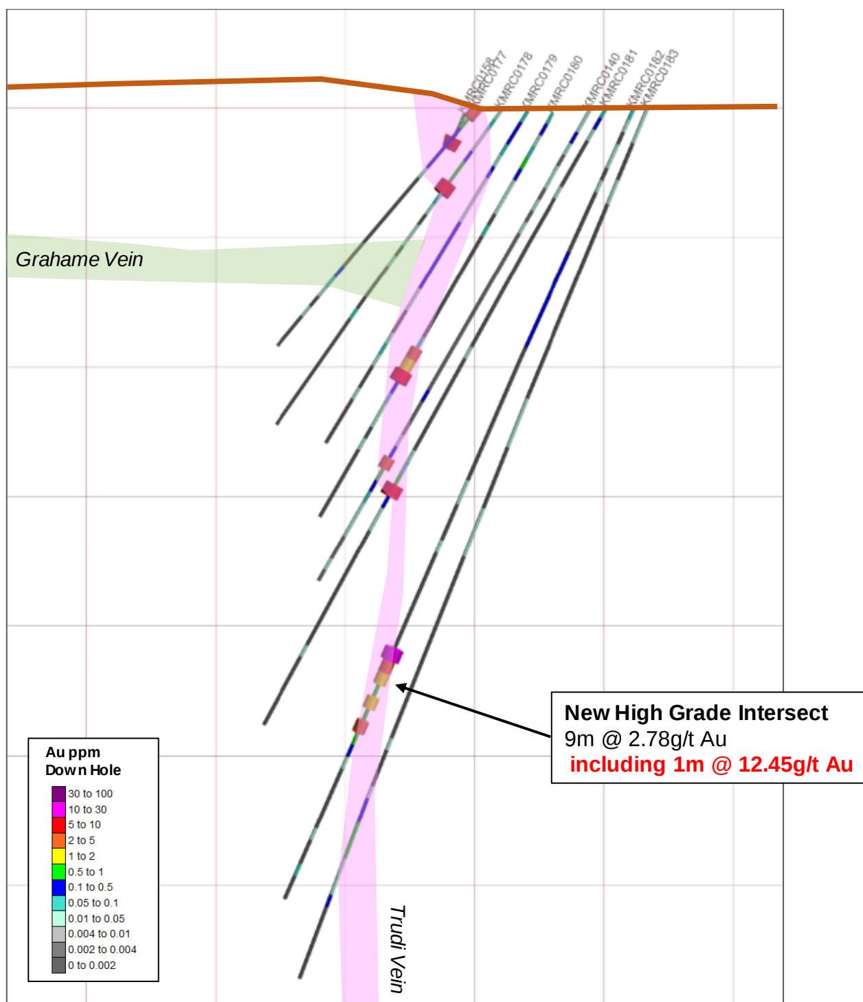
Figure 4 Results on 359009mE section looking west
