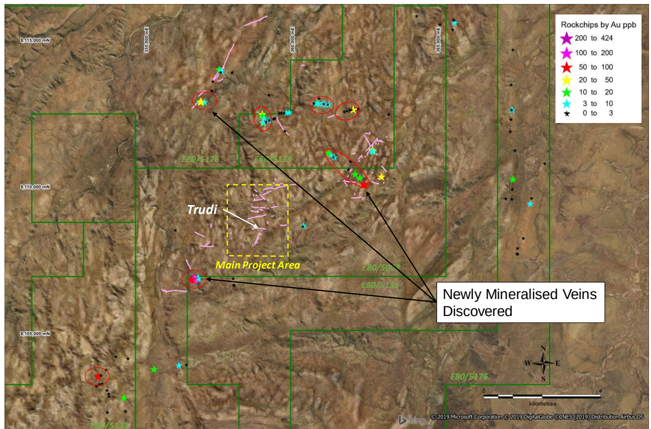
Figure 3: Location of recently discovered mineralised veins (red ovals) outside the main project area.
