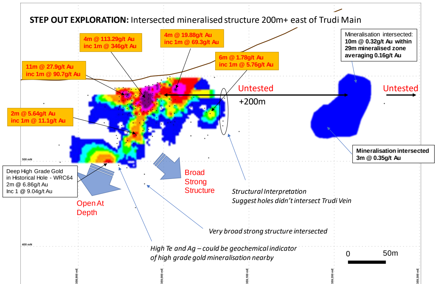
Figure 2: Long projection, looking north, showing the Trudi Main area and possible extensions to the east.
