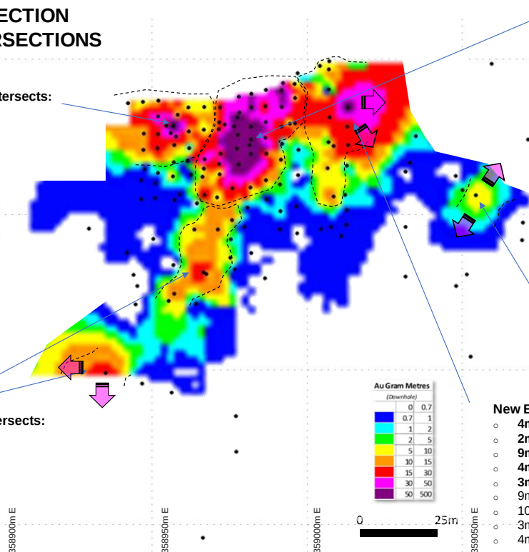
Figure 1: Long projection, looking north, showing the multiple very high-grade gold results from the Trudi Main Area. Best results labelled (previously announced).
