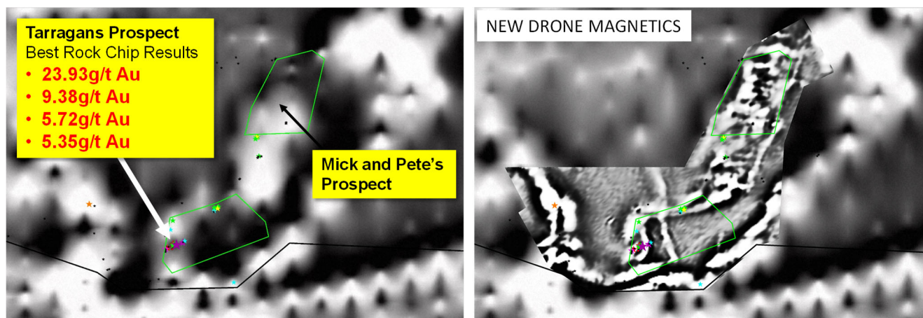
Figure 6: Tennant East Project area magnetics (black and white) and gravity (coloured) with main target areas. Best rock chip results previously reported (KRR ASX release 8/3/23).
