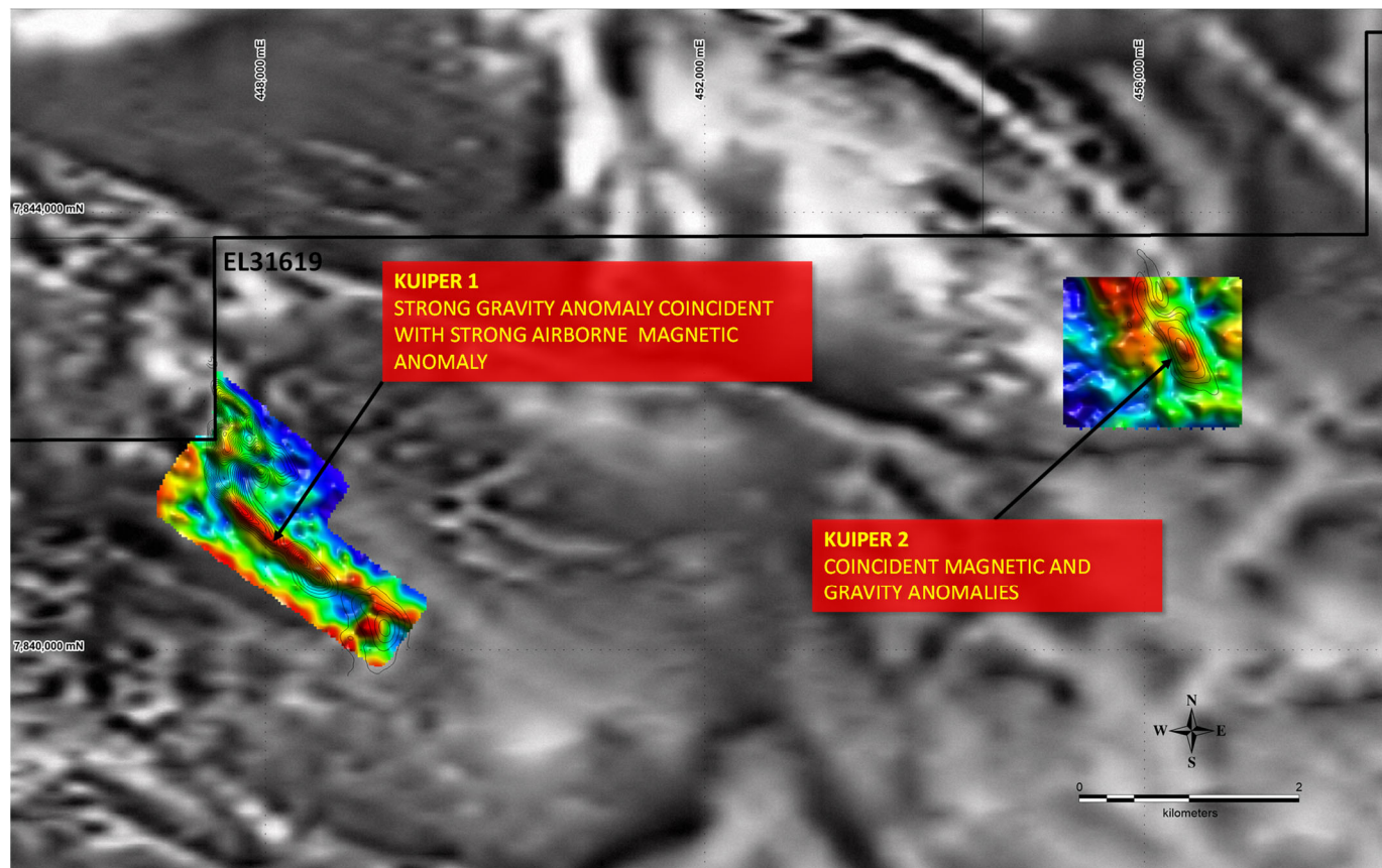
Figure 4: Gravity survey results for Kuiper targets, Tennant East, residual gravity as coloured images over 1vd magnetics, black contours highlight airborne magnetic high targets.
